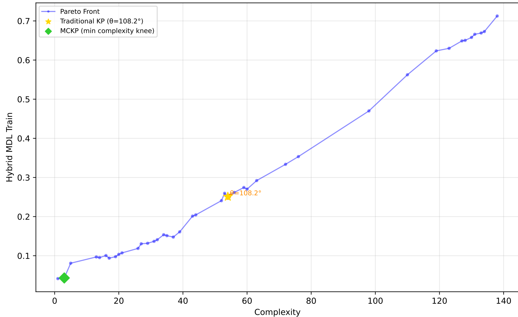
522_pm10 - Run 25 - MVP - Hybrid MDL Train \lambda_1=1.00, \lambda_2=0.00, \lambda_3=0.00 | Difficulty: 0.97 | Method: hmr
