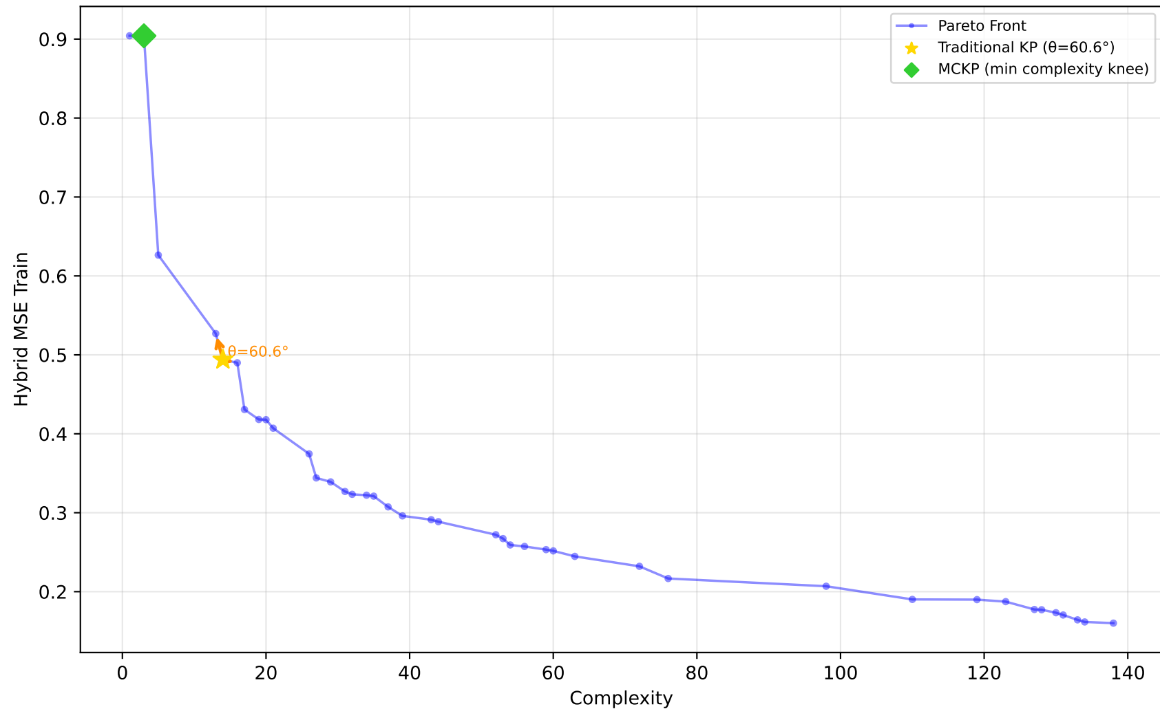
522_pm10 - Run 25 - MVP - Hybrid MSE Train \lambda_1=0.00, \lambda_2=0.90, \lambda_3=0.00 | Difficulty: 0.97 | Method: hmr
