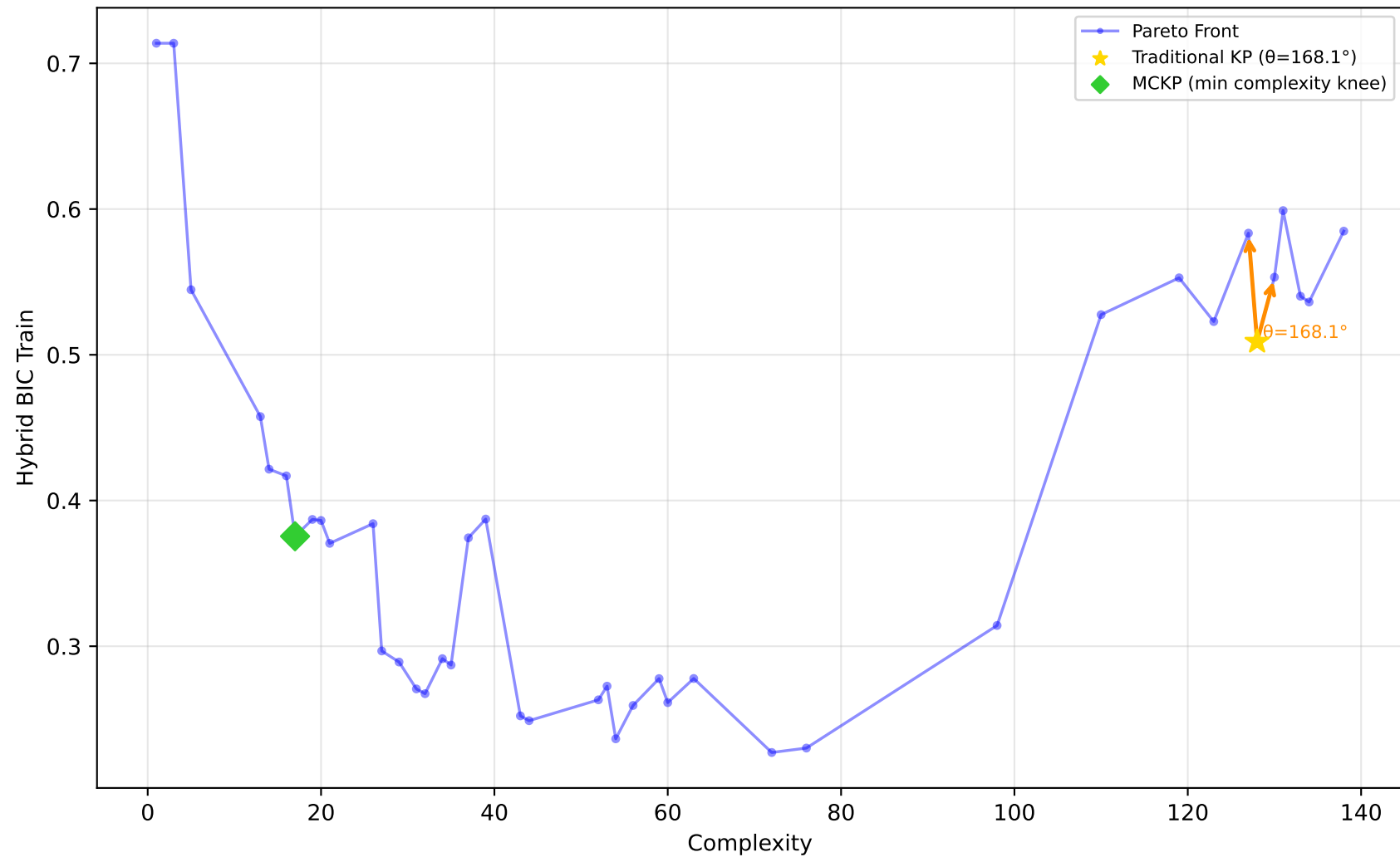
522_pm10 - Run 25 - SVP - Hybrid BIC Train \lambda_1=1.00, \lambda_2=0.00, \lambda_3=0.90 | Difficulty: 0.97 | Method: hmr
