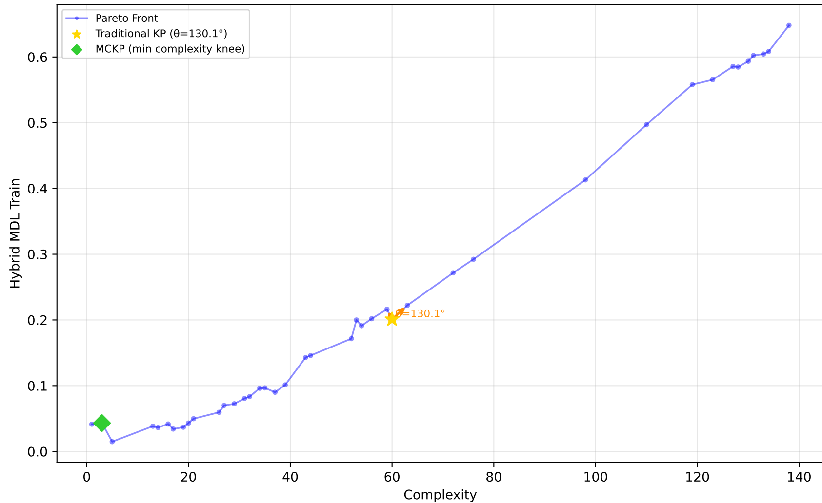
522_pm10 - Run 25 - SVP - Hybrid MDL Train \lambda_1=0.00, \lambda_2=0.10, \lambda_3=0.00 | Difficulty: 0.97 | Method: hmr
