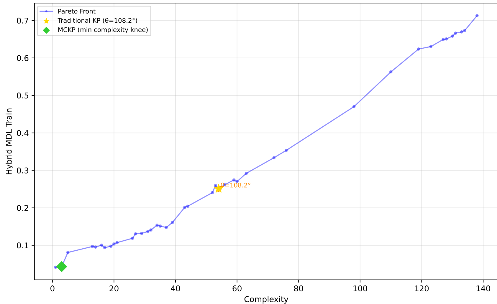
522_pm10 - Run 25 - SVP - Hybrid MDL Train \lambda_1=1.00, \lambda_2=0.00, \lambda_3=0.90 | Difficulty: 0.97 | Method: hmr
