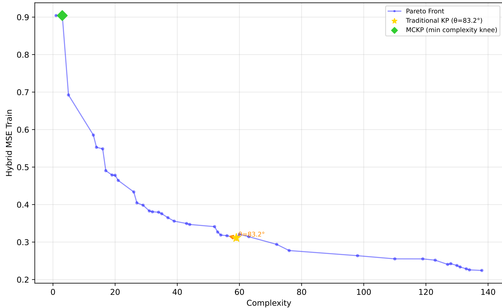
522_pm10 - Run 25 - SVP - Hybrid MSE Train \lambda_1=1.00, \lambda_2=0.00, \lambda_3=0.90 | Difficulty: 0.97 | Method: hmr
