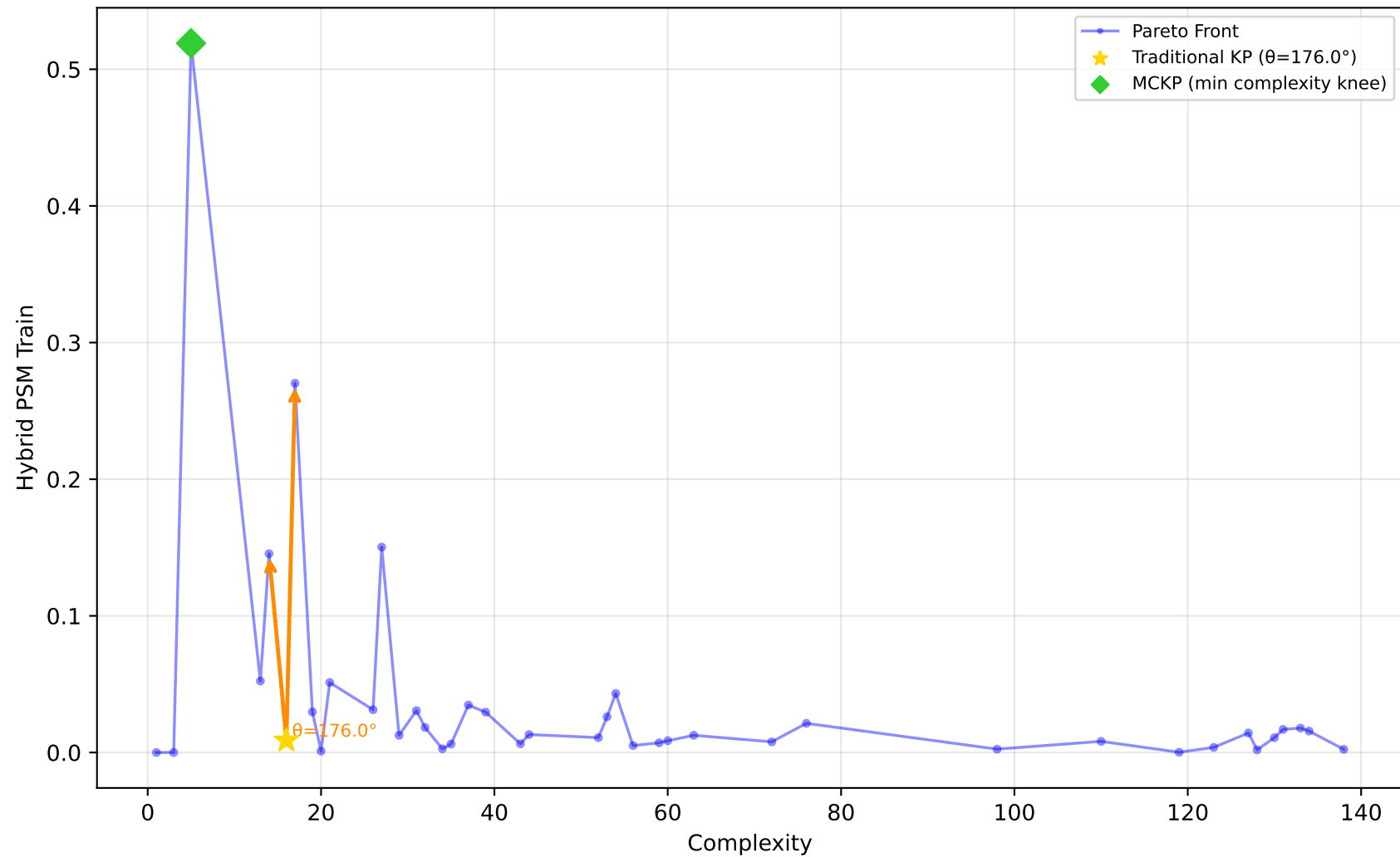
522_pm10 - Run 25 - SVP - Hybrid PSM Train \lambda_1=0.00, \lambda_2=0.10, \lambda_3=0.00 | Difficulty: 0.97 | Method: hmr
