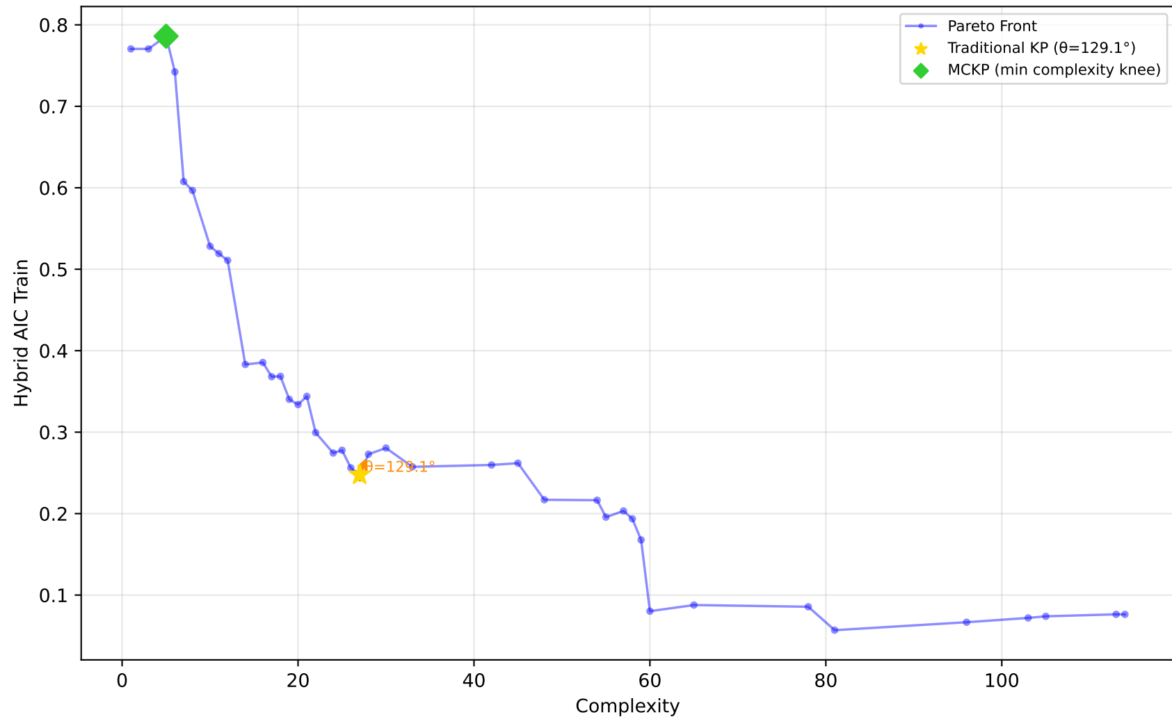
522_pm10 - Run 26 - MVP - Hybrid AIC Train \lambda_1=1.00, \lambda_2=0.00, \lambda_3=0.00 | Difficulty: 1.00 | Method: hmr
