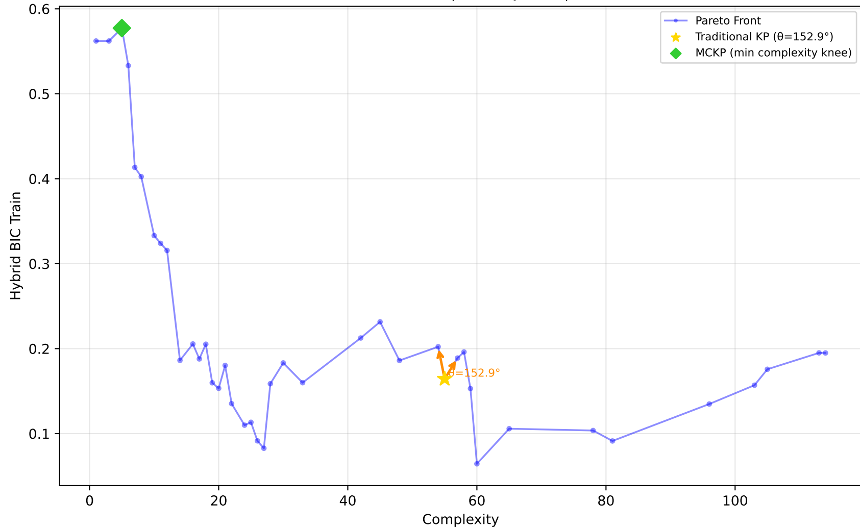
522_pm10 - Run 26 - MVP - Hybrid BIC Train \lambda_1=1.00, \lambda_2=0.00, \lambda_3=0.00 | Difficulty: 1.00 | Method: hmr
