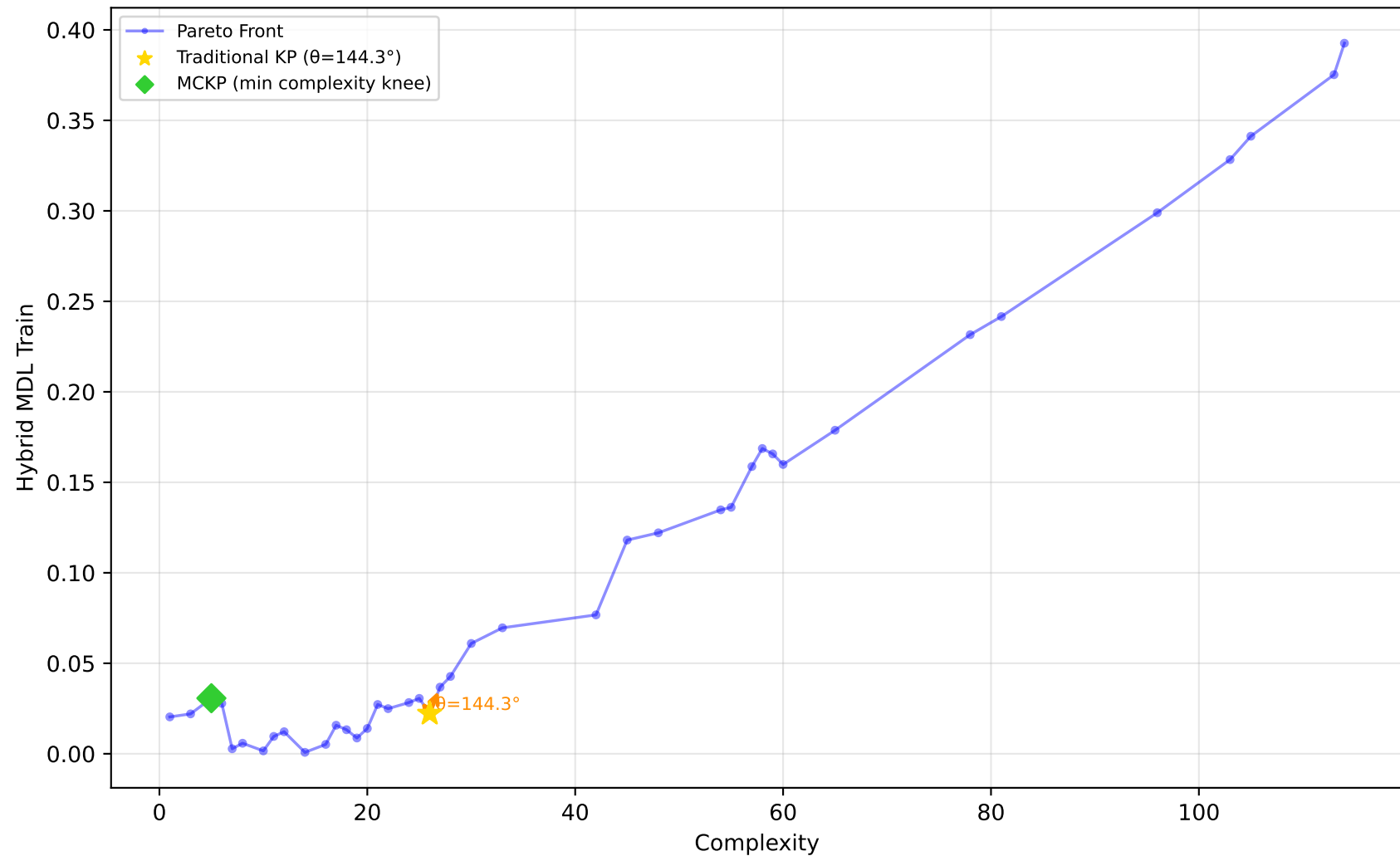
522_pm10 - Run 26 - MVP - Hybrid MDL Train \lambda_1=0.00, \lambda_2=0.90, \lambda_3=0.00 | Difficulty: 1.00 | Method: hmr
