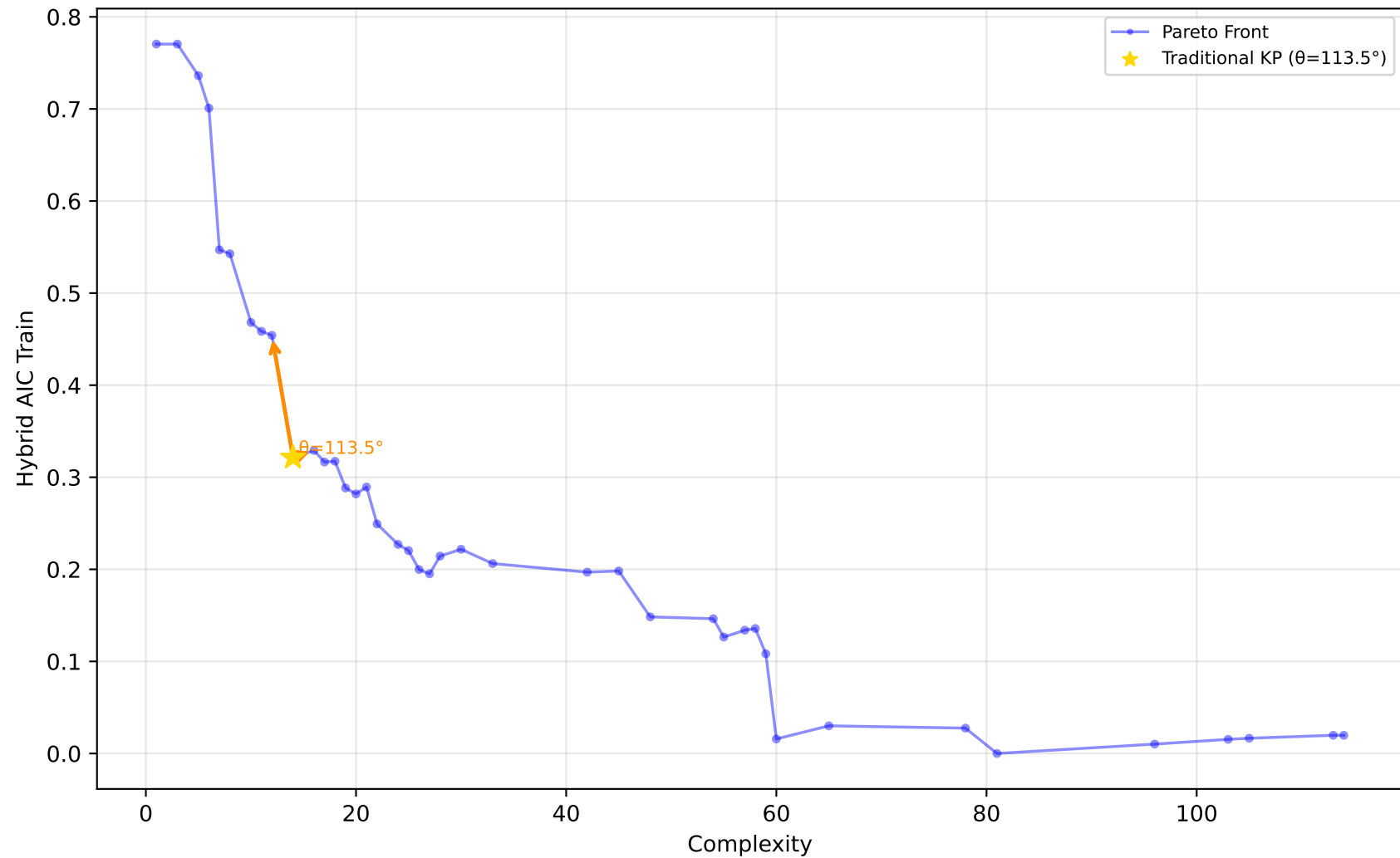
522_pm10 - Run 26 - SVP - Hybrid AIC Train \lambda_1=0.00, \lambda_2=0.10, \lambda_3=0.00 | Difficulty: 1.00 | Method: hmr
