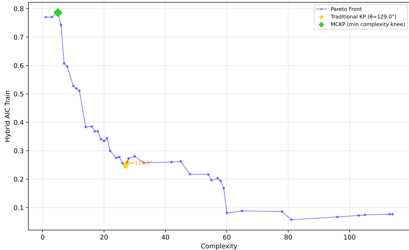
522_pm10 - Run 26 - SVP - Hybrid AIC Train \lambda_1=1.00, \lambda_2=0.00, \lambda_3=0.90 | Difficulty: 1.00 | Method: hmr
