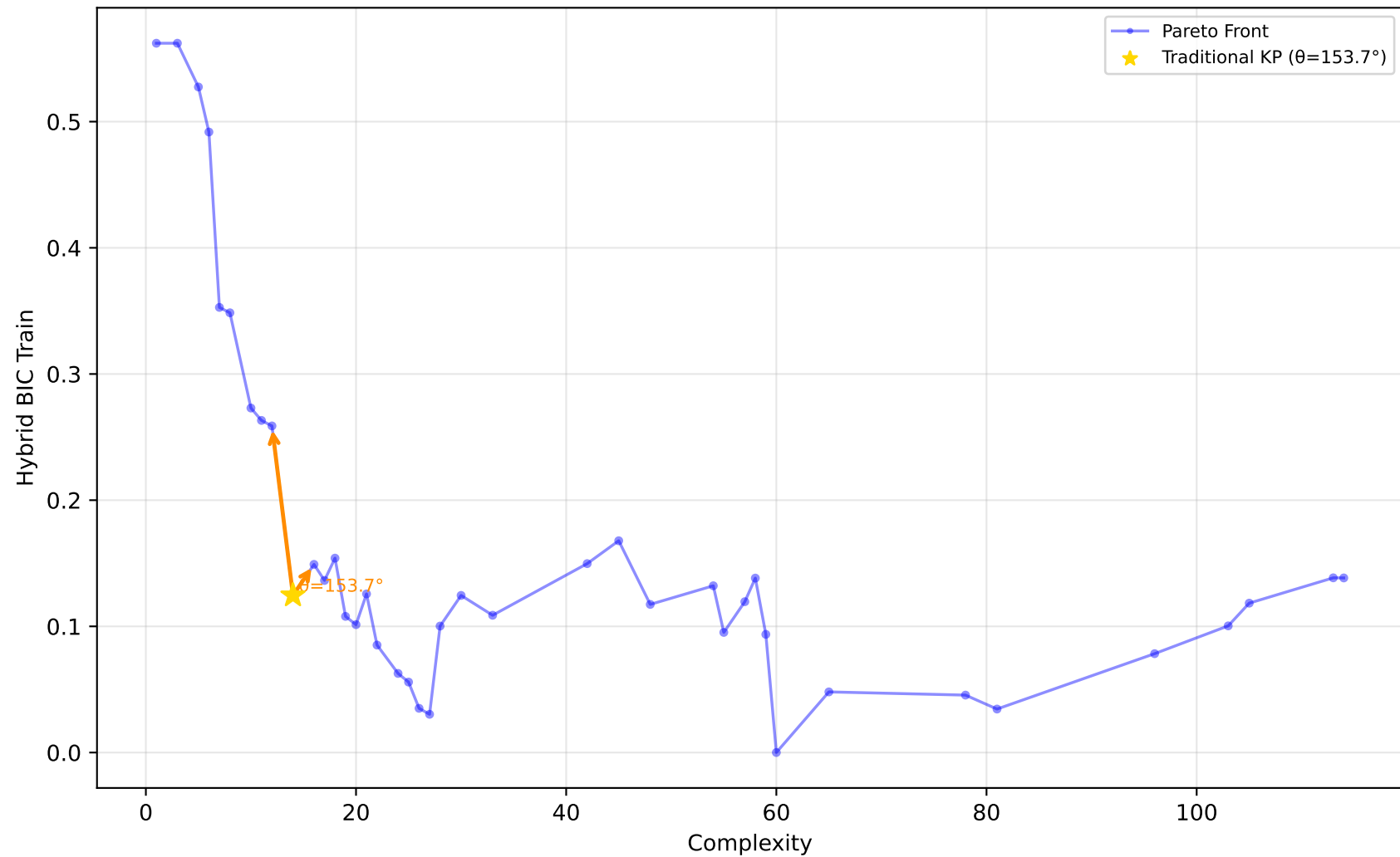
522_pm10 - Run 26 - SVP - Hybrid BIC Train \lambda_1=0.00, \lambda_2=0.10, \lambda_3=0.00 | Difficulty: 1.00 | Method: hmr
