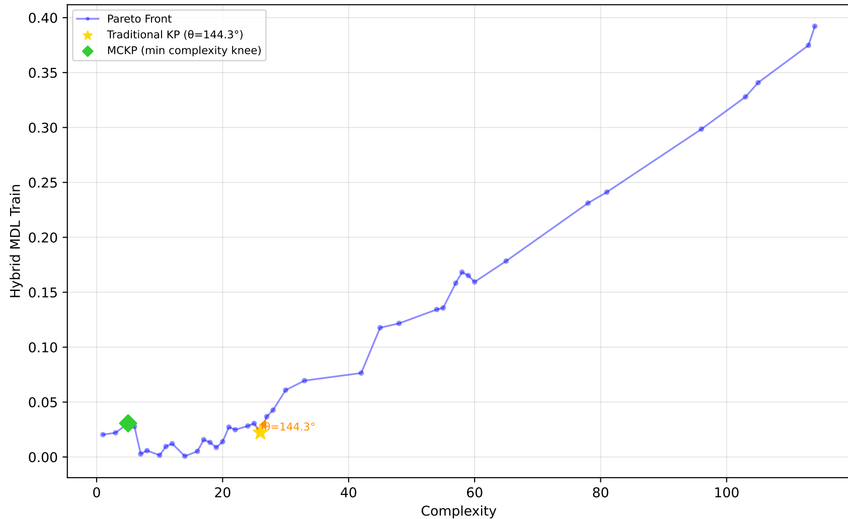
522_pm10 - Run 26 - SVP - Hybrid MDL Train \lambda_1=0.00, \lambda_2=0.10, \lambda_3=0.00 | Difficulty: 1.00 | Method: hmr
