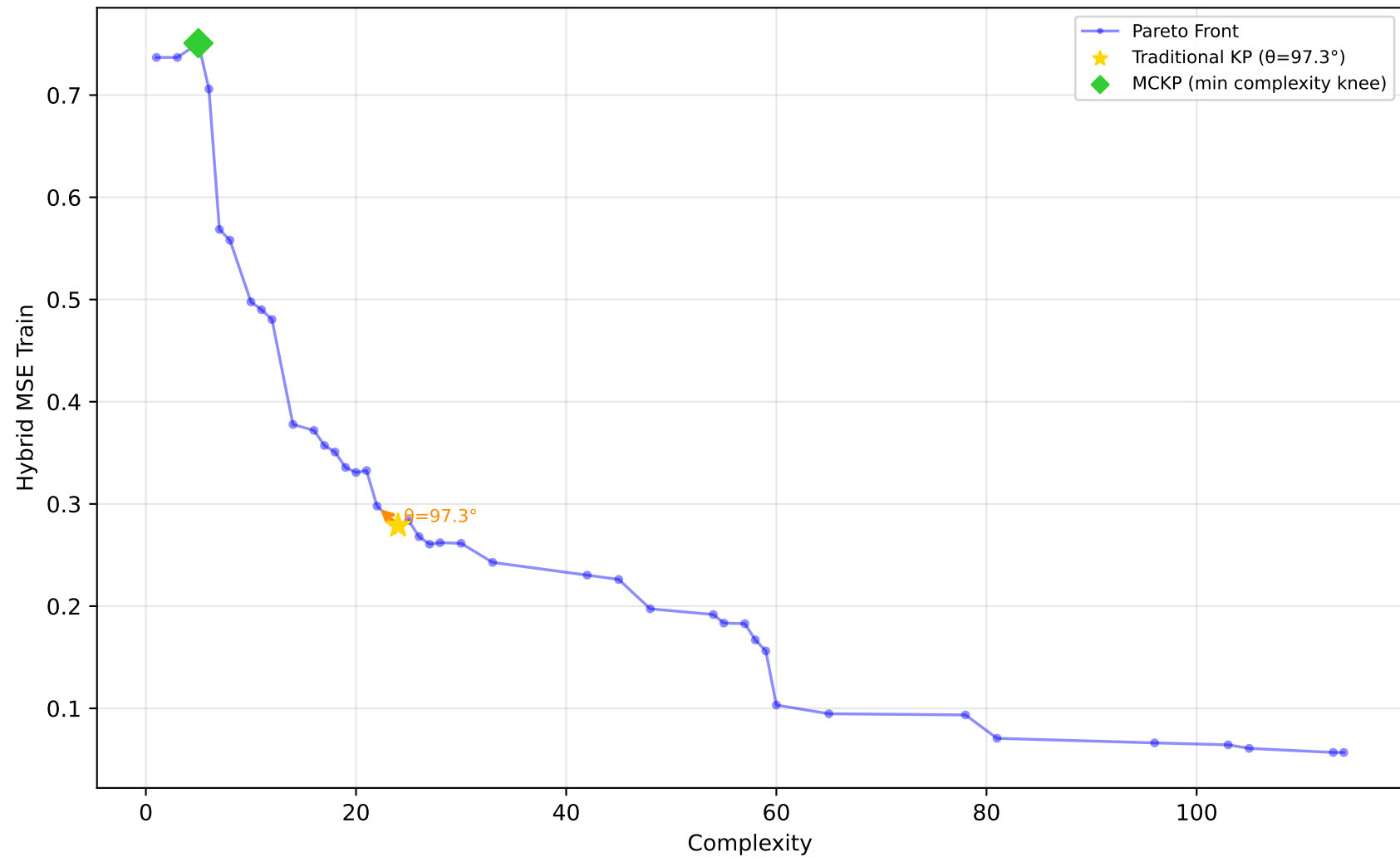
522_pm10 - Run 26 - SVP - Hybrid MSE Train \lambda_1=1.00, \lambda_2=0.00, \lambda_3=0.90 | Difficulty: 1.00 | Method: hmr
