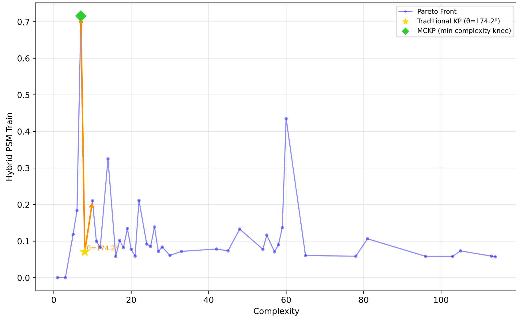
522_pm10 - Run 26 - SVP - Hybrid PSM Train \lambda_1=1.00, \lambda_2=0.00, \lambda_3=0.90 | Difficulty: 1.00 | Method: hmr
