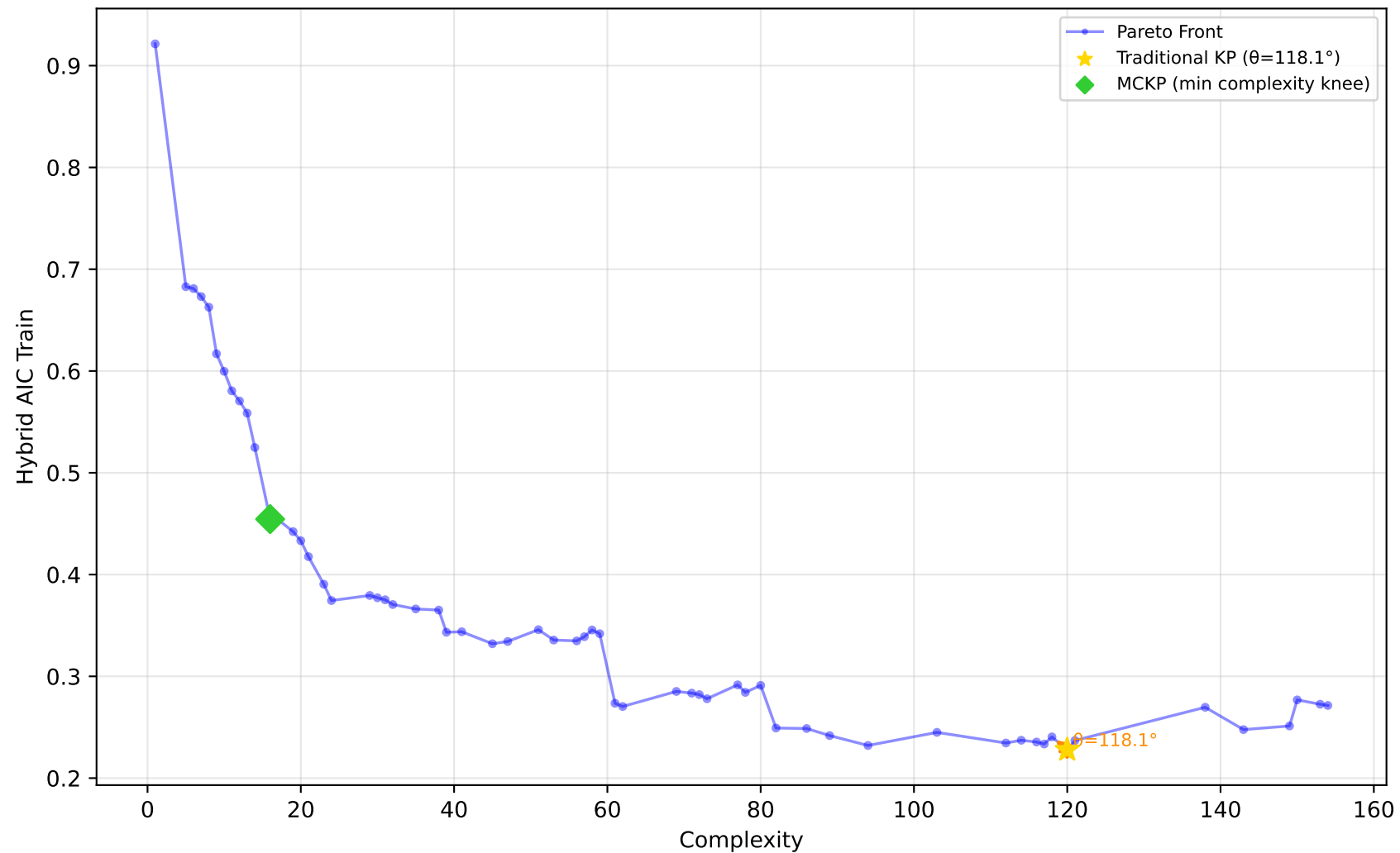
522_pm10 - Run 27 - MVP - Hybrid AIC Train \lambda_1=0.00, \lambda_2=0.90, \lambda_3=0.00 | Difficulty: 1.00 | Method: hmr
