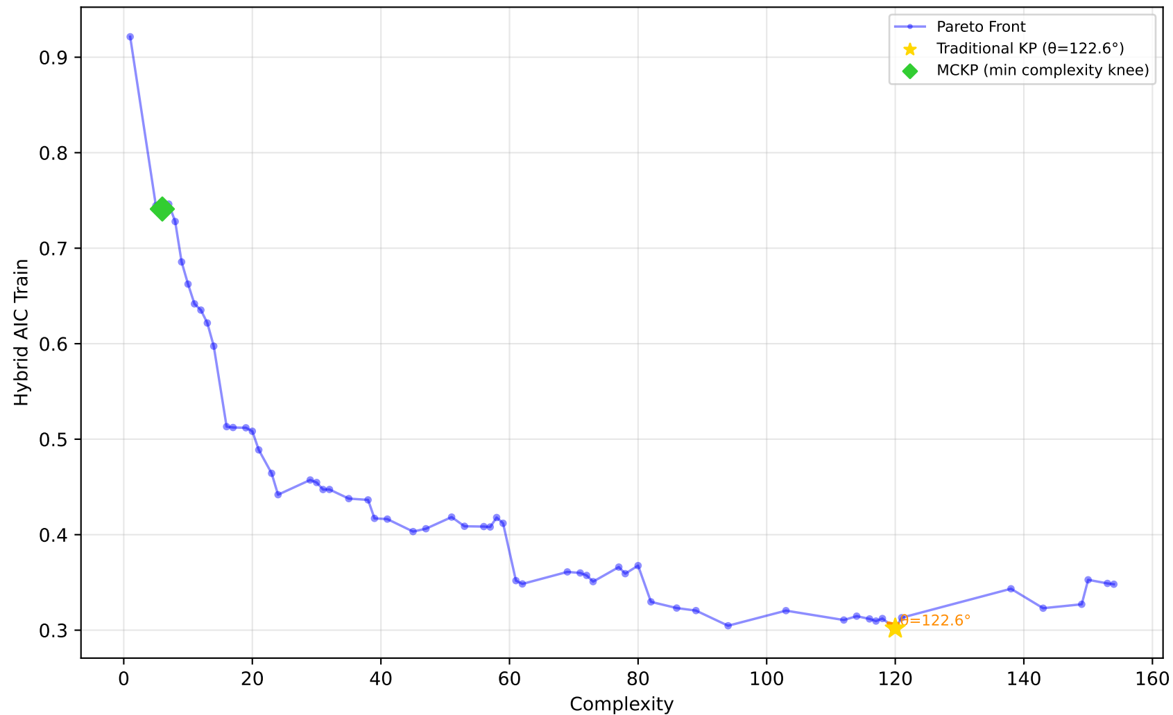
522_pm10 - Run 27 - MVP - Hybrid AIC Train \lambda_1=1.00, \lambda_2=0.00, \lambda_3=0.00 | Difficulty: 1.00 | Method: hmr
