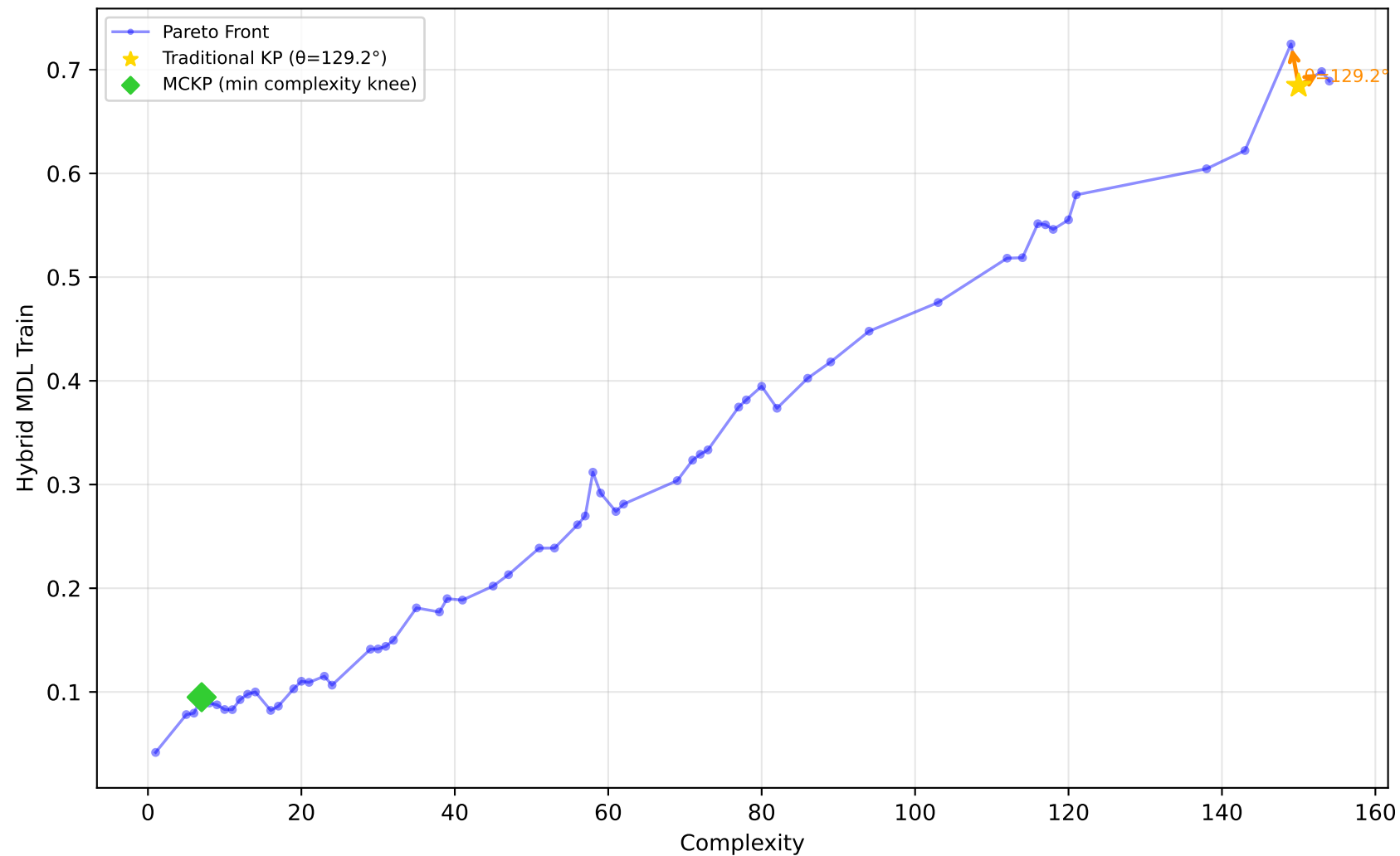
522_pm10 - Run 27 - MVP - Hybrid MDL Train \lambda_1=1.00, \lambda_2=0.00, \lambda_3=0.00 | Difficulty: 1.00 | Method: hmr
