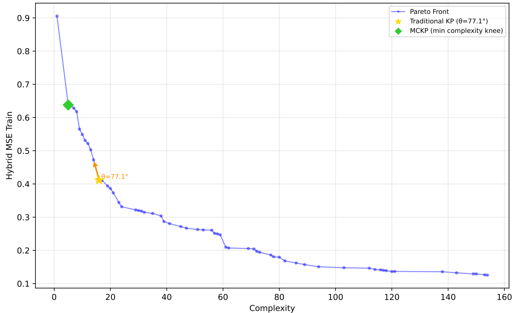
522_pm10 - Run 27 - MVP - Hybrid MSE Train \lambda_1=0.00, \lambda_2=0.90, \lambda_3=0.00 | Difficulty: 1.00 | Method: hmr
