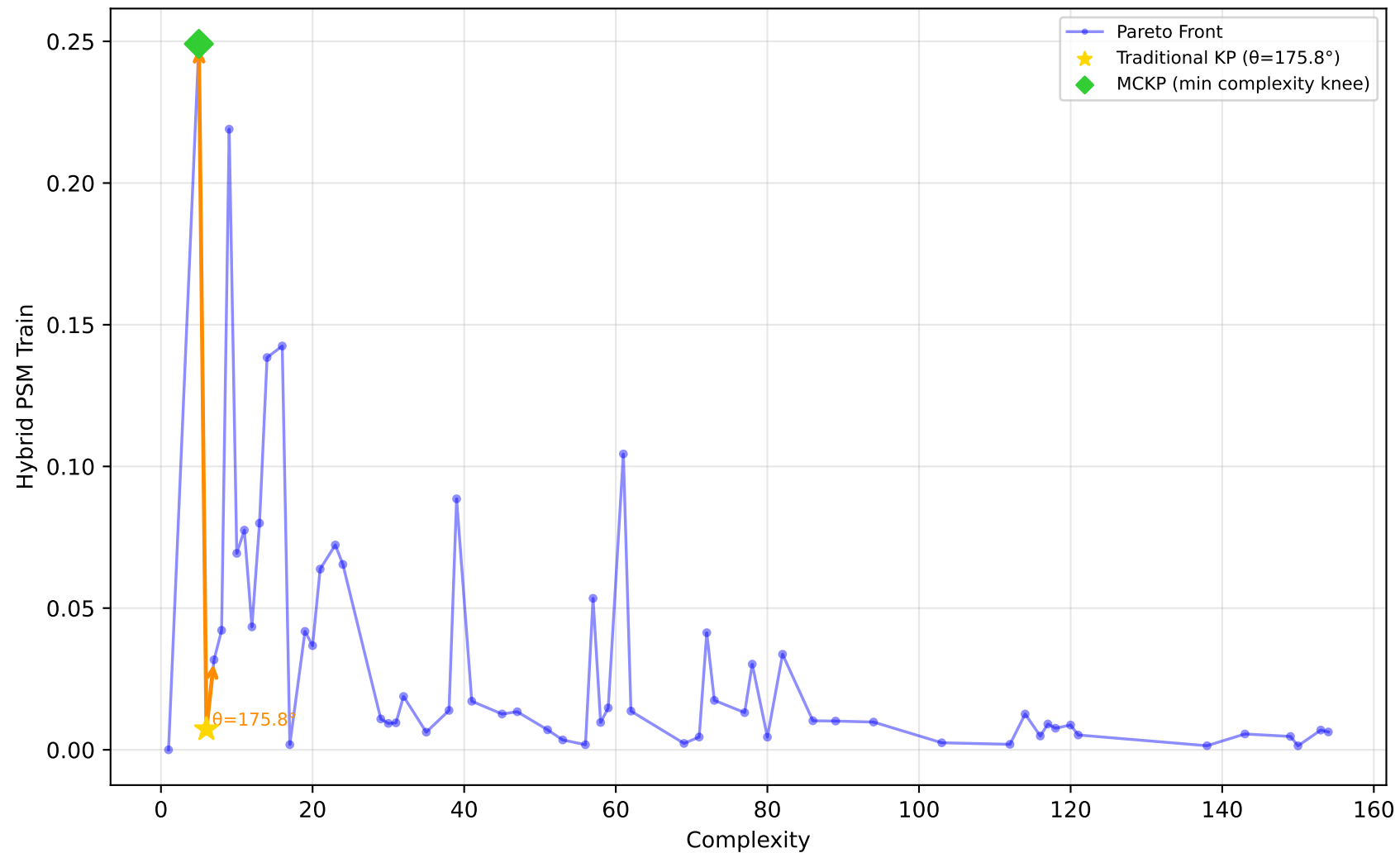
522_pm10 - Run 27 - MVP - Hybrid PSM Train \lambda_1=0.00 , \lambda_2=0.90 , \lambda_3=0.00 | Difficulty: 1.00 | Method: hmr
