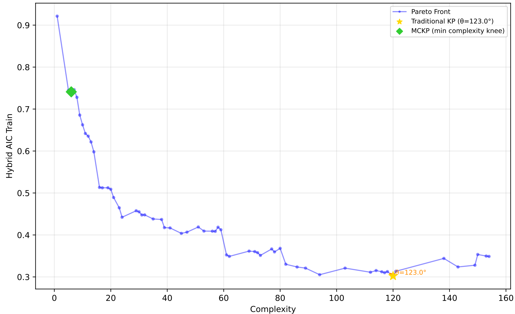
522_pm10 - Run 27 - SVP - Hybrid AIC Train \lambda_1=1.00, \lambda_2=0.00, \lambda_3=0.90 | Difficulty: 1.00 | Method: hmr
