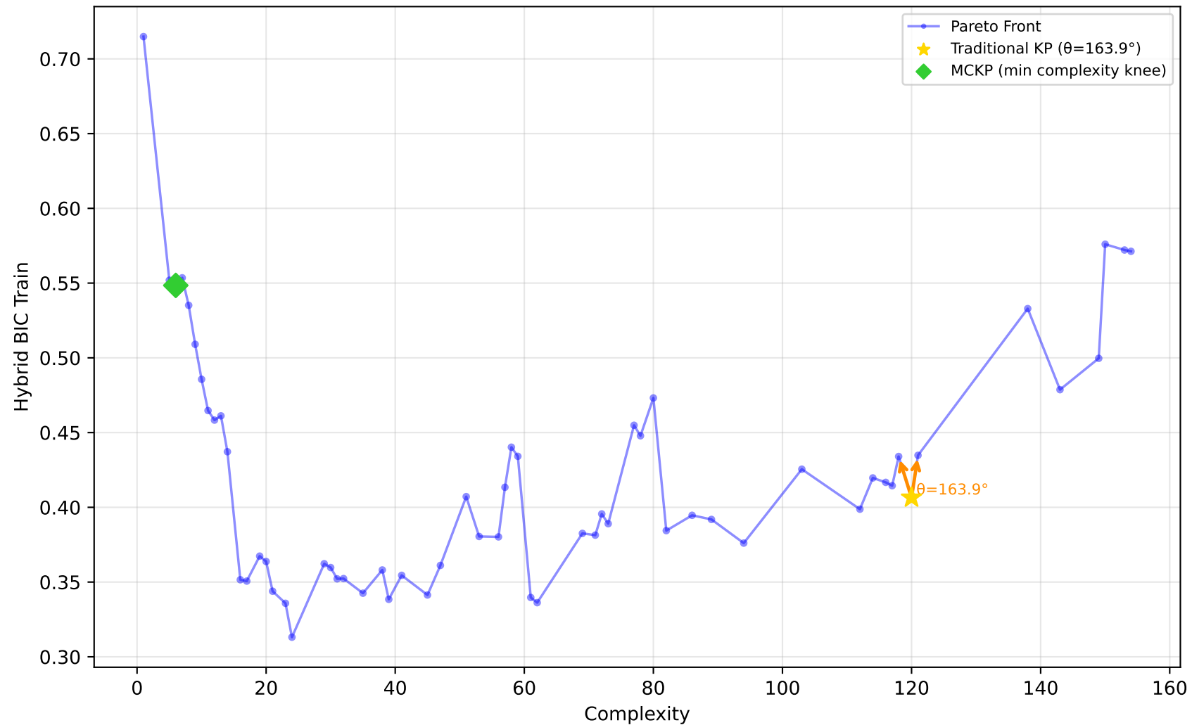
522_pm10 - Run 27 - SVP - Hybrid BIC Train \lambda_1=1.00 , \lambda_2=0.00 , \lambda_3=0.90 | Difficulty: 1.00 | Method: hmr
