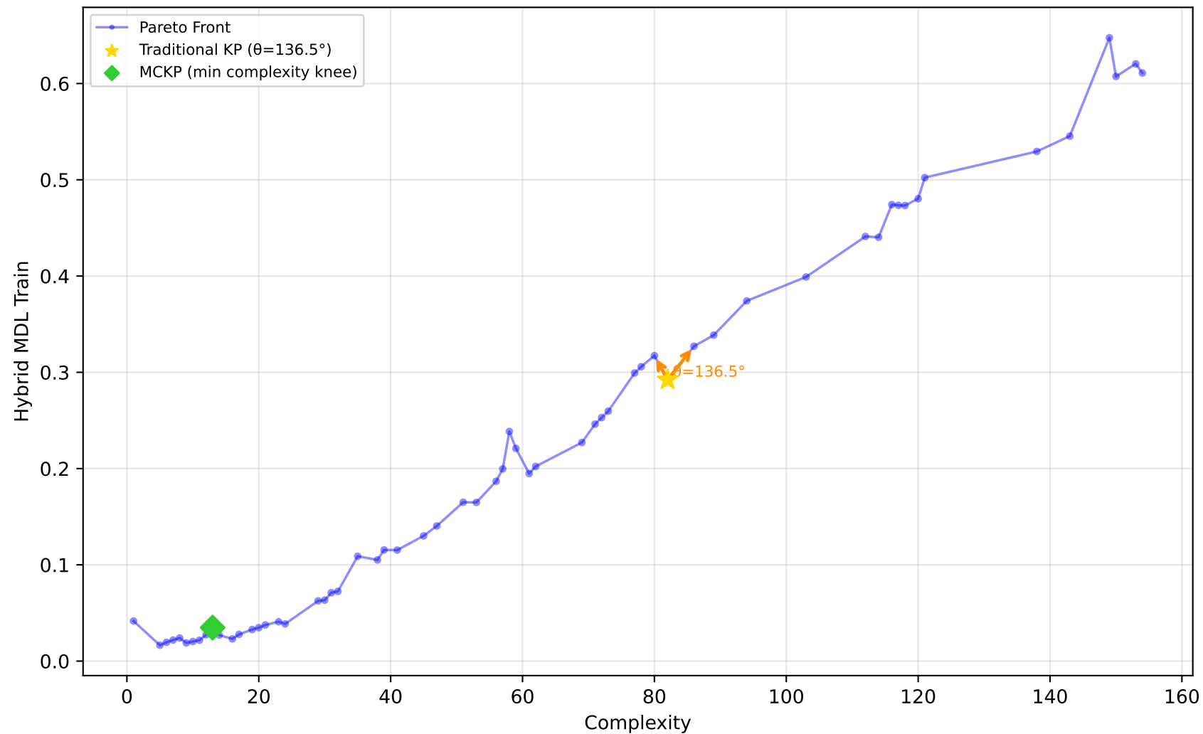
522_pm10 - Run 27 - SVP - Hybrid MDL Train \lambda_1=0.00, \lambda_2=0.10, \lambda_3=0.00 | Difficulty: 1.00 | Method: hmr
