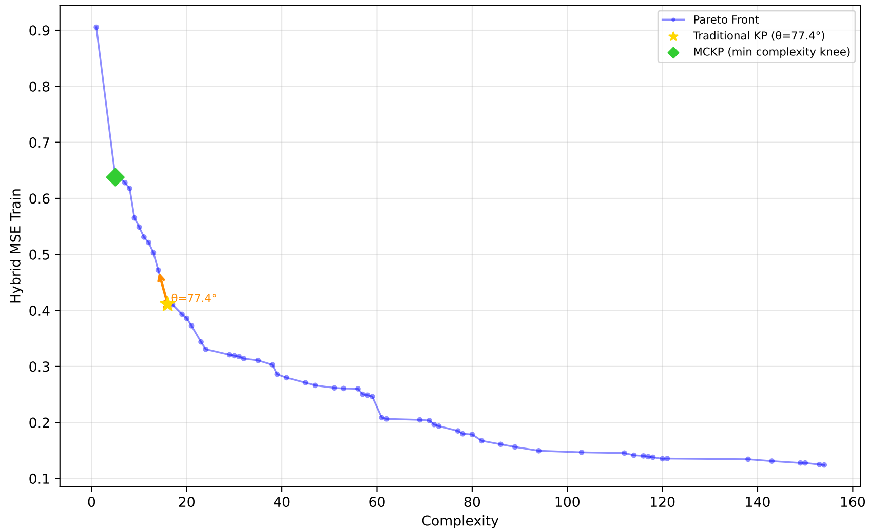
522_pm10 - Run 27 - SVP - Hybrid MSE Train \lambda_1=0.00, \lambda_2=0.10, \lambda_3=0.00 | Difficulty: 1.00 | Method: hmr
