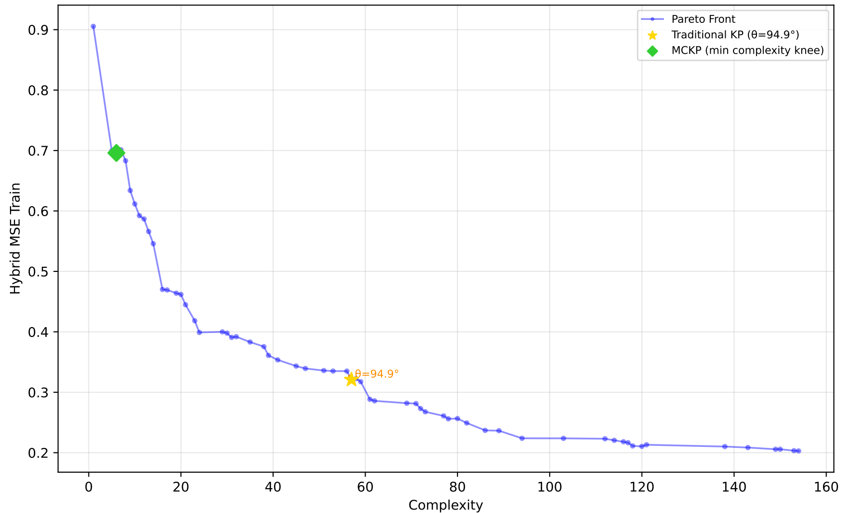
522_pm10 - Run 27 - SVP - Hybrid MSE Train \lambda_1=1.00, \lambda_2=0.00, \lambda_3=0.90 | Difficulty: 1.00 | Method: hmr
