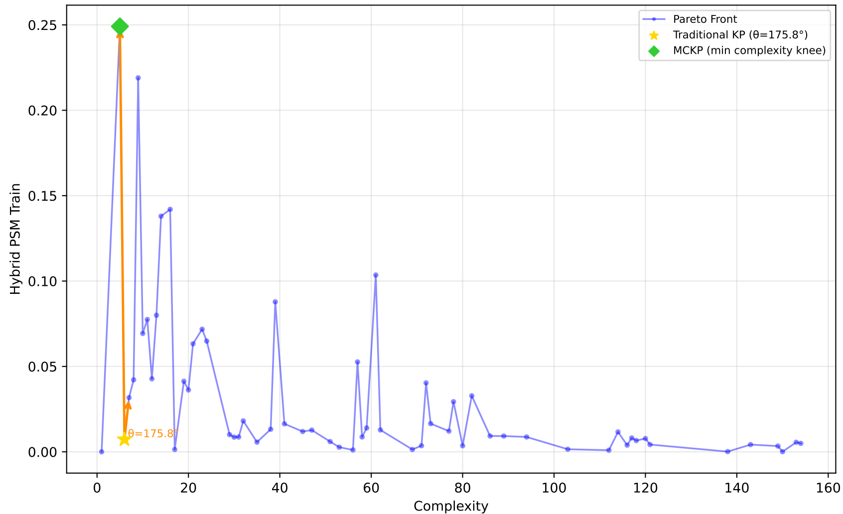
522_pm10 - Run 27 - SVP - Hybrid PSM Train \lambda_1=0.00 , \lambda_2=0.10 , \lambda_3=0.00 | Difficulty: 1.00 | Method: hmr
