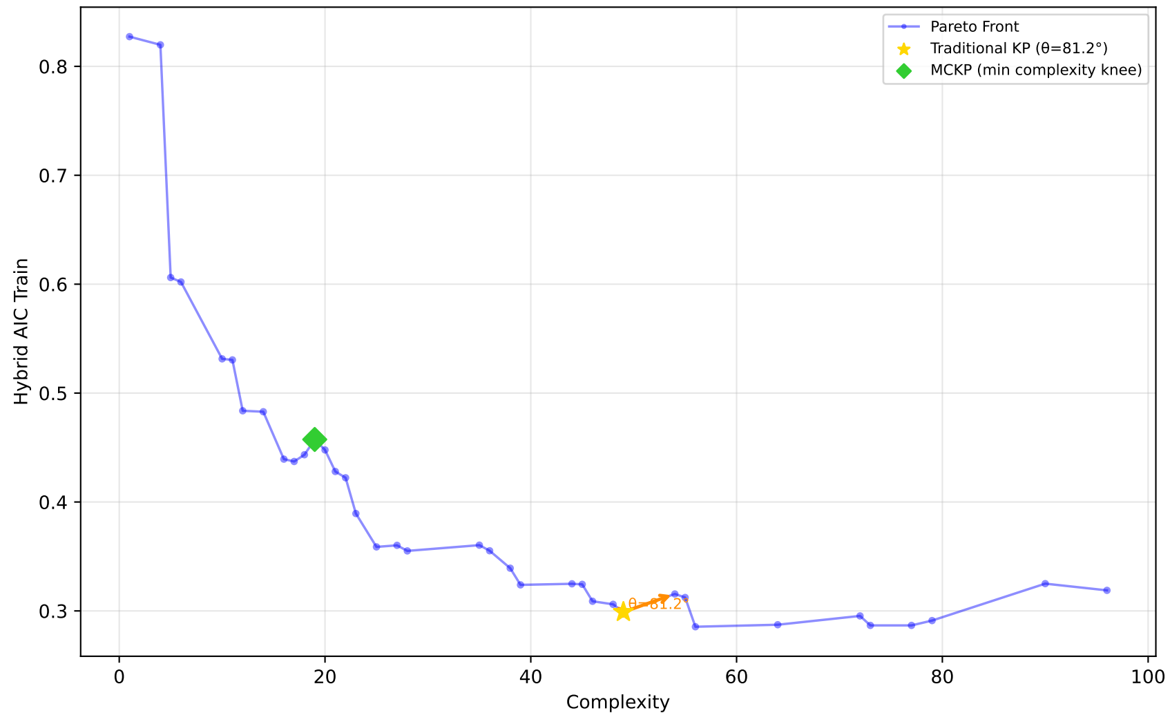
522_pm10 - Run 28 - MVP - Hybrid AIC Train \lambda_1=0.00, \lambda_2=0.90, \lambda_3=0.00 | Difficulty: 1.00 | Method: hmr
