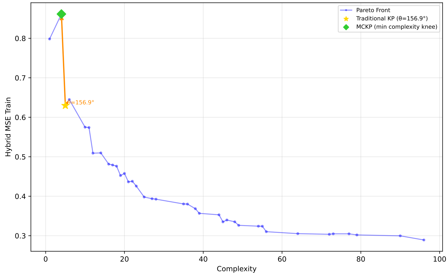
522_pm10 - Run 28 - MVP - Hybrid MSE Train \lambda_1=1.00, \lambda_2=0.00, \lambda_3=0.00 | Difficulty: 1.00 | Method: hmr
