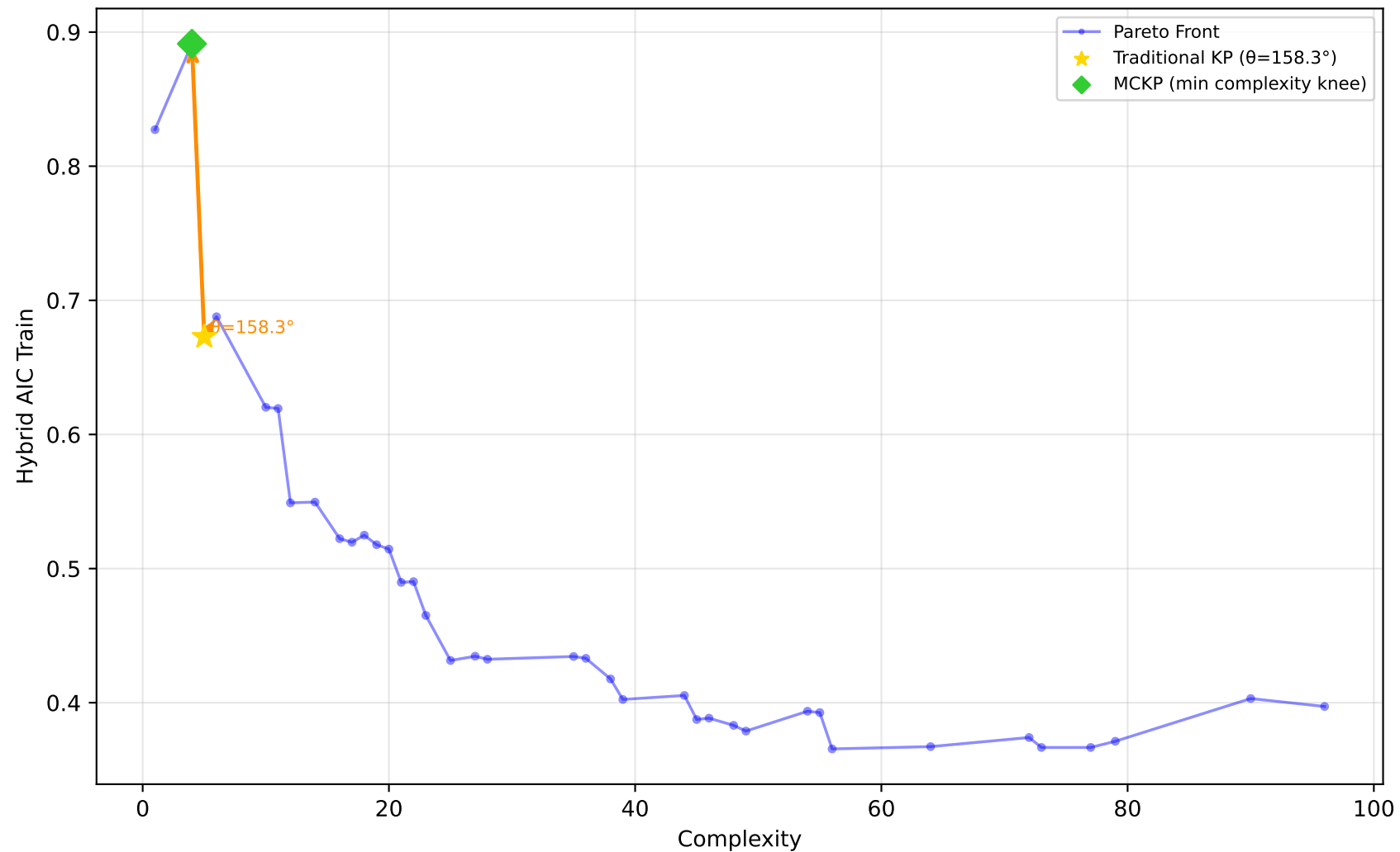
522_pm10 - Run 28 - SVP - Hybrid AIC Train \lambda_1=1.00, \lambda_2=0.00, \lambda_3=0.90 | Difficulty: 1.00 | Method: hmr
