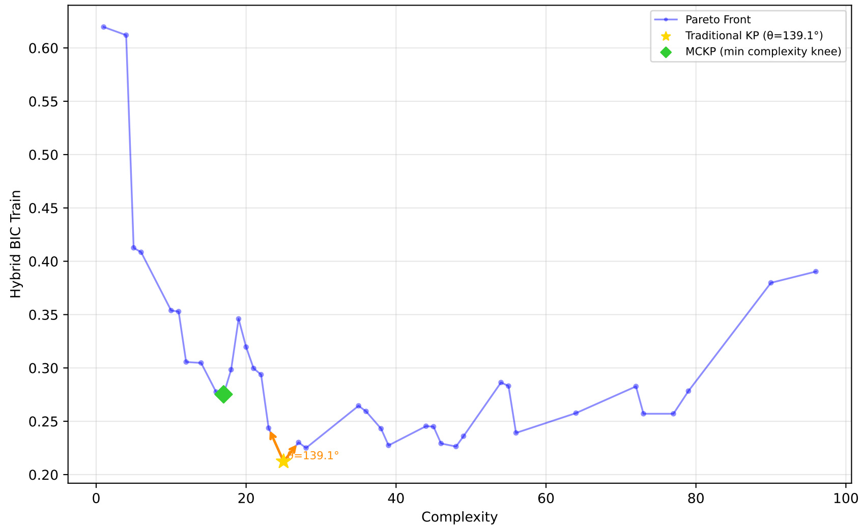
522_pm10 - Run 28 - SVP - Hybrid BIC Train \lambda_1=0.00, \lambda_2=0.10, \lambda_3=0.00 | Difficulty: 1.00 | Method: hmr
