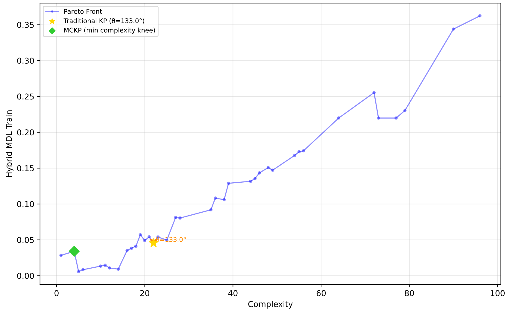
522_pm10 - Run 28 - SVP - Hybrid MDL Train \lambda_1=0.00, \lambda_2=0.10, \lambda_3=0.00 | Difficulty: 1.00 | Method: hmr
