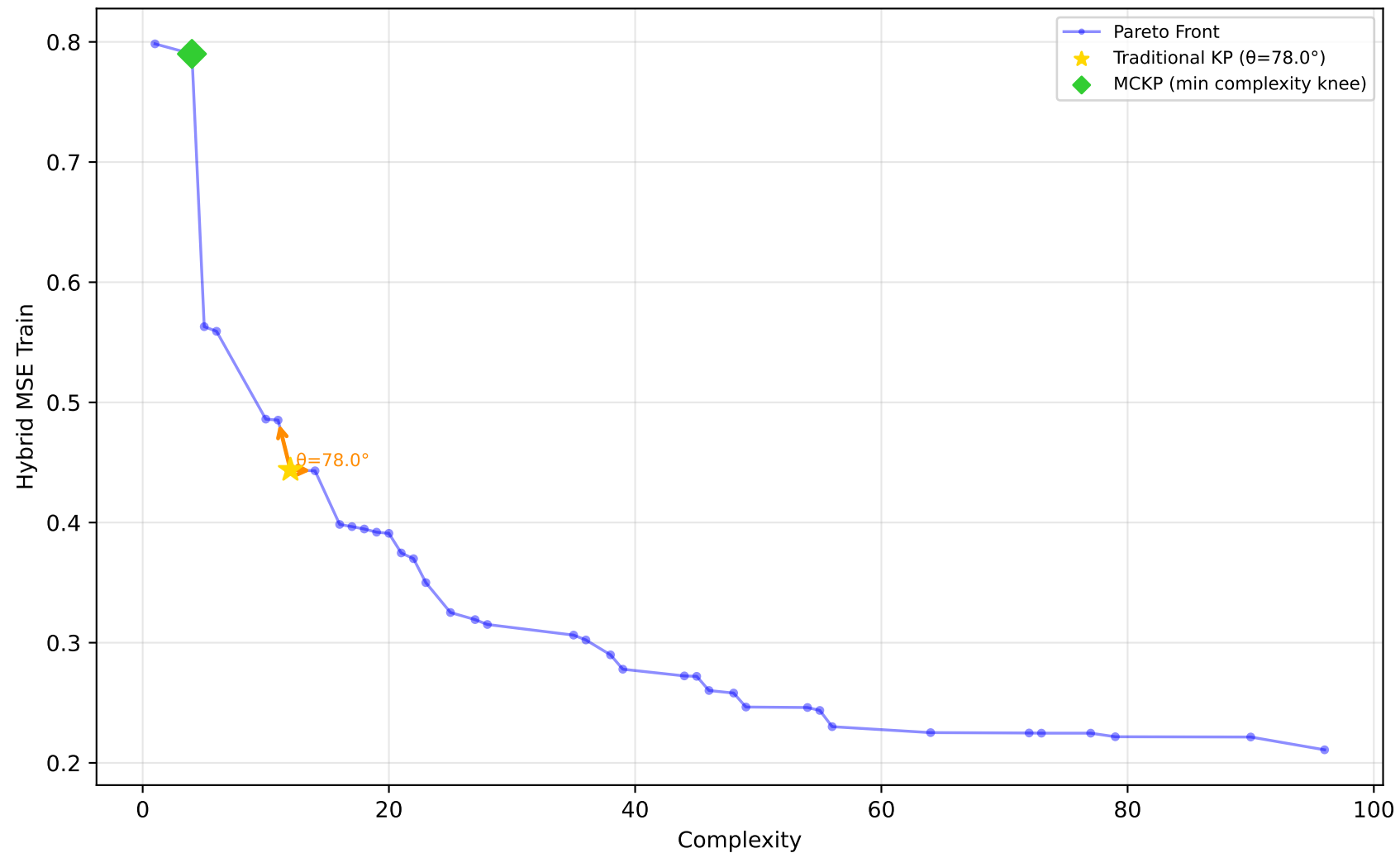
522_pm10 - Run 28 - SVP - Hybrid MSE Train \lambda_1=0.00, \lambda_2=0.10, \lambda_3=0.00 | Difficulty: 1.00 | Method: hmr
