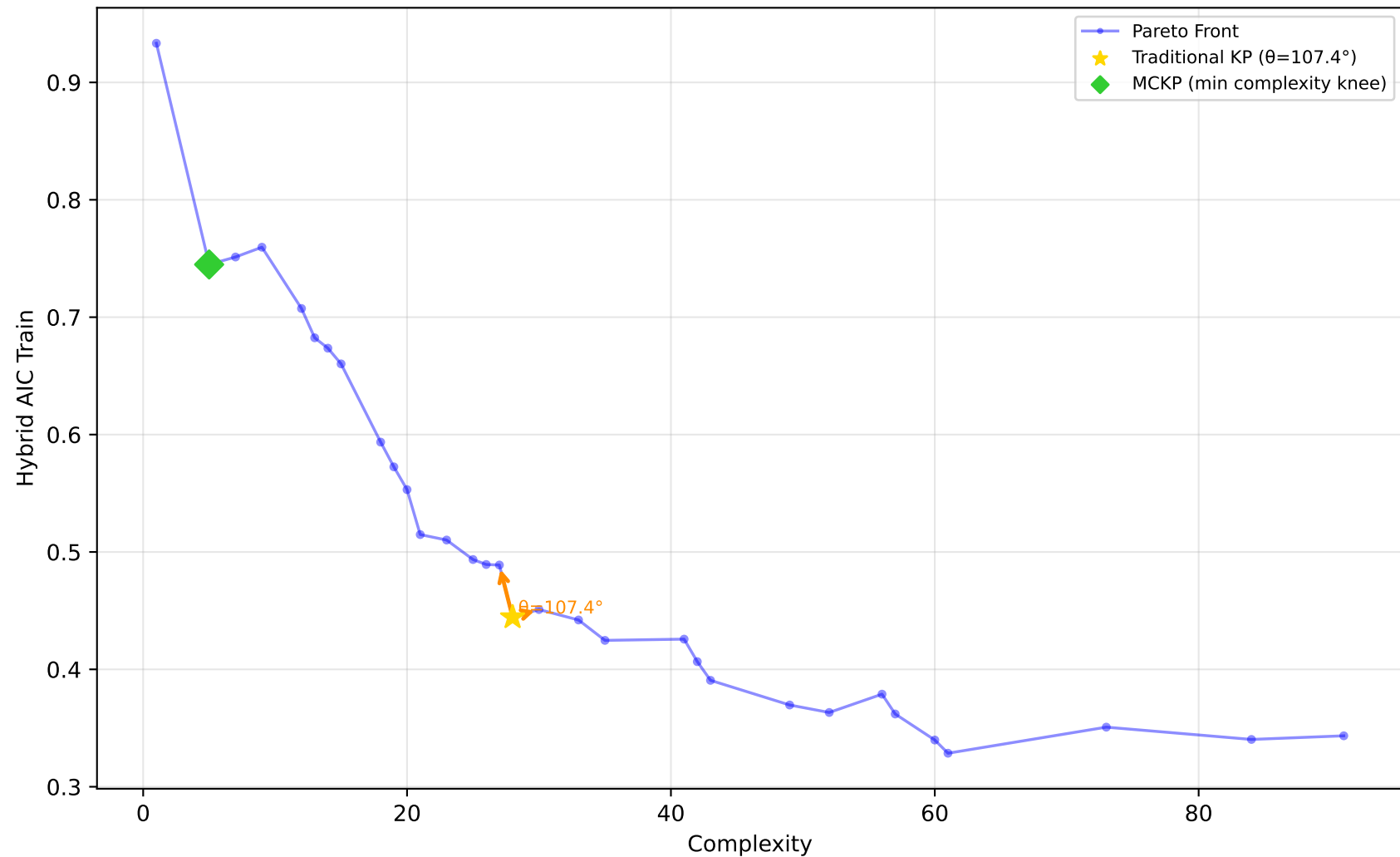
522_pm10 - Run 29 - MVP - Hybrid AIC Train \lambda_1=0.00, \lambda_2=0.90, \lambda_3=0.00 | Difficulty: 1.00 | Method: hmr
