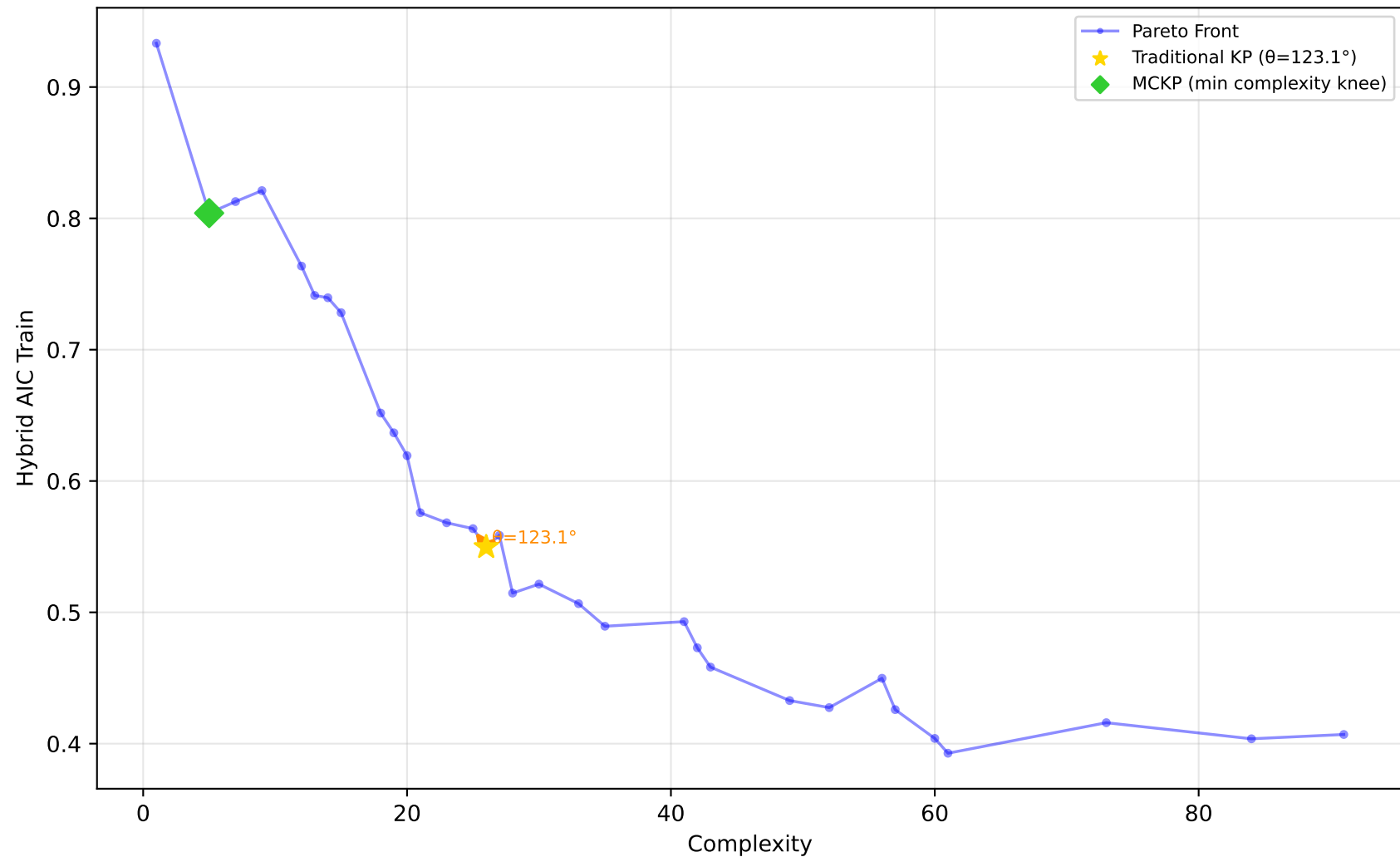
522_pm10 - Run 29 - SVP - Hybrid AIC Train \lambda_1=1.00, \lambda_2=0.00, \lambda_3=0.90 | Difficulty: 1.00 | Method: hmr
