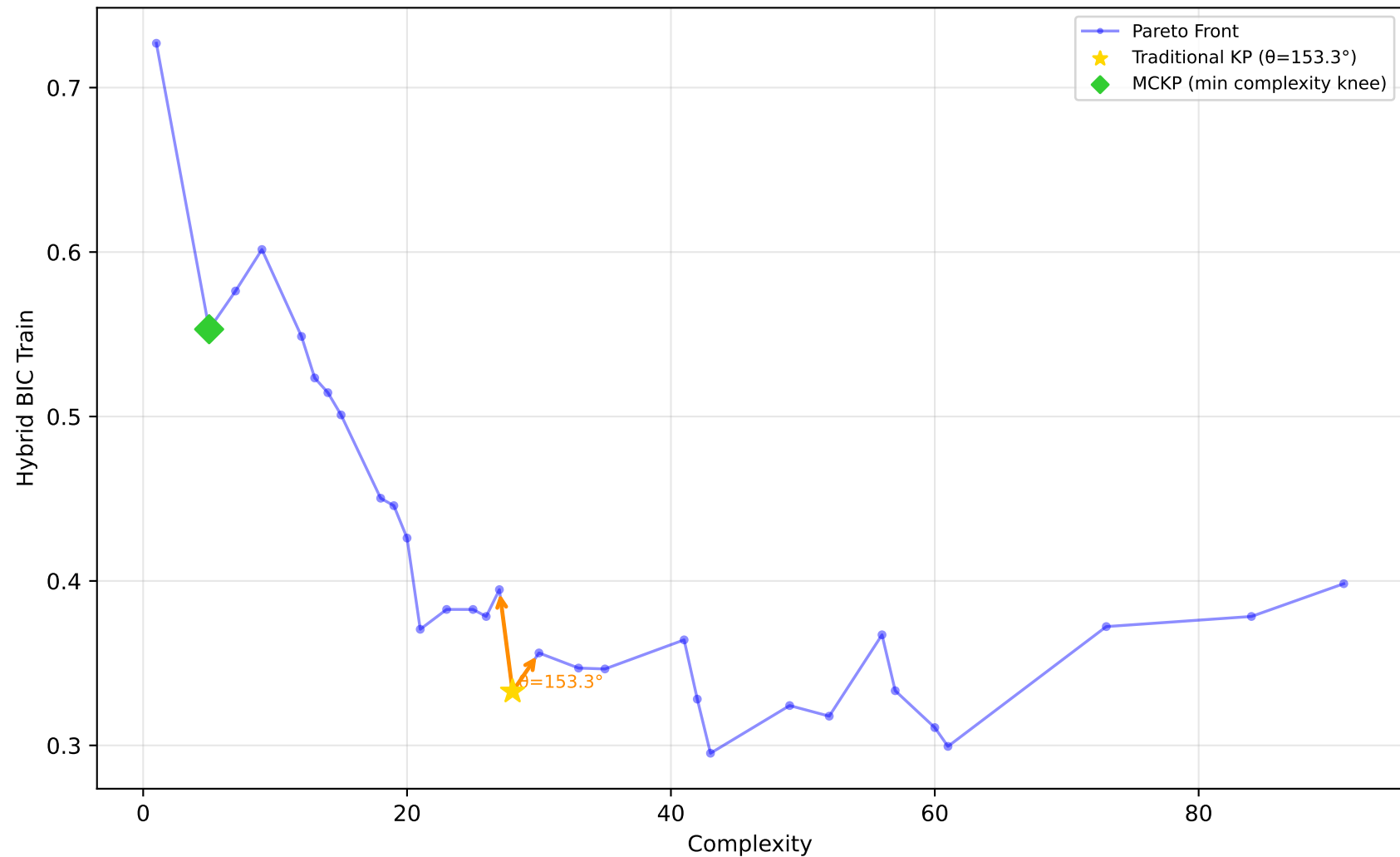
522_pm10 - Run 29 - SVP - Hybrid BIC Train \lambda_1=0.00, \lambda_2=0.10, \lambda_3=0.00 | Difficulty: 1.00 | Method: hmr
