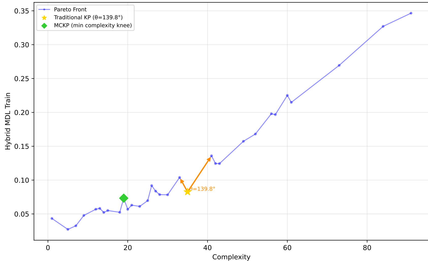
522_pm10 - Run 29 - SVP - Hybrid MDL Train \lambda_1=0.00, \lambda_2=0.10, \lambda_3=0.00 | Difficulty: 1.00 | Method: hmr
