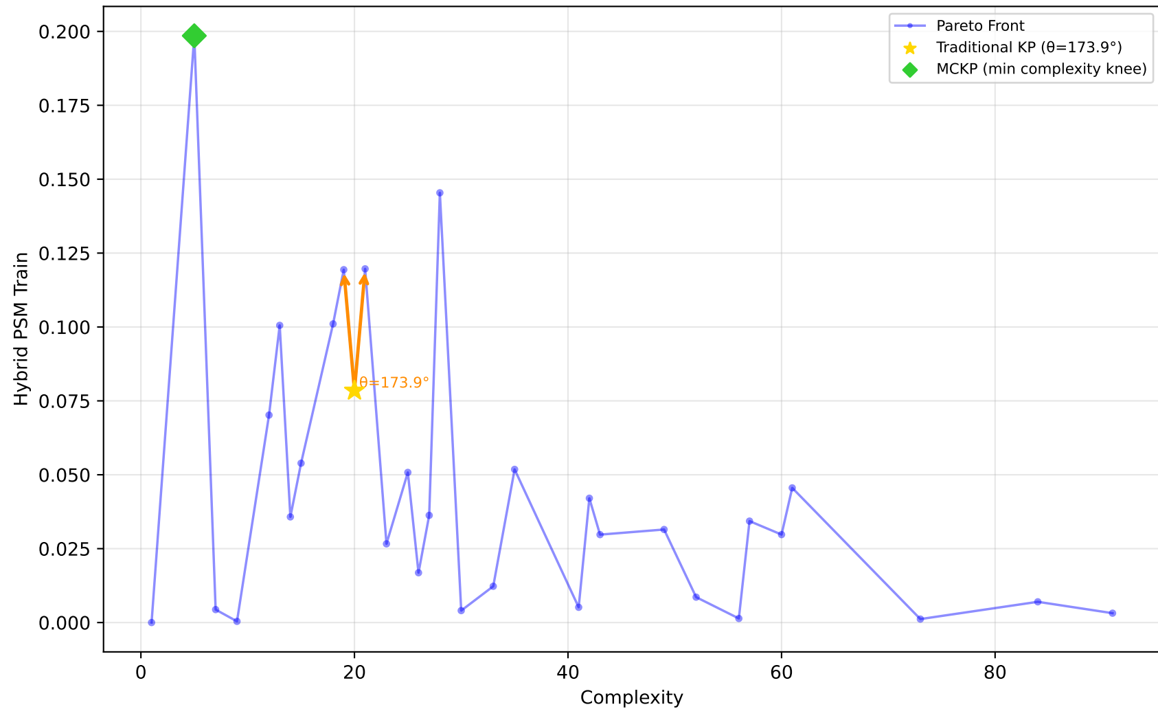
522_pm10 - Run 29 - SVP - Hybrid PSM Train \lambda_1=0.00, \lambda_2=0.10, \lambda_3=0.00 | Difficulty: 1.00 | Method: hmr
