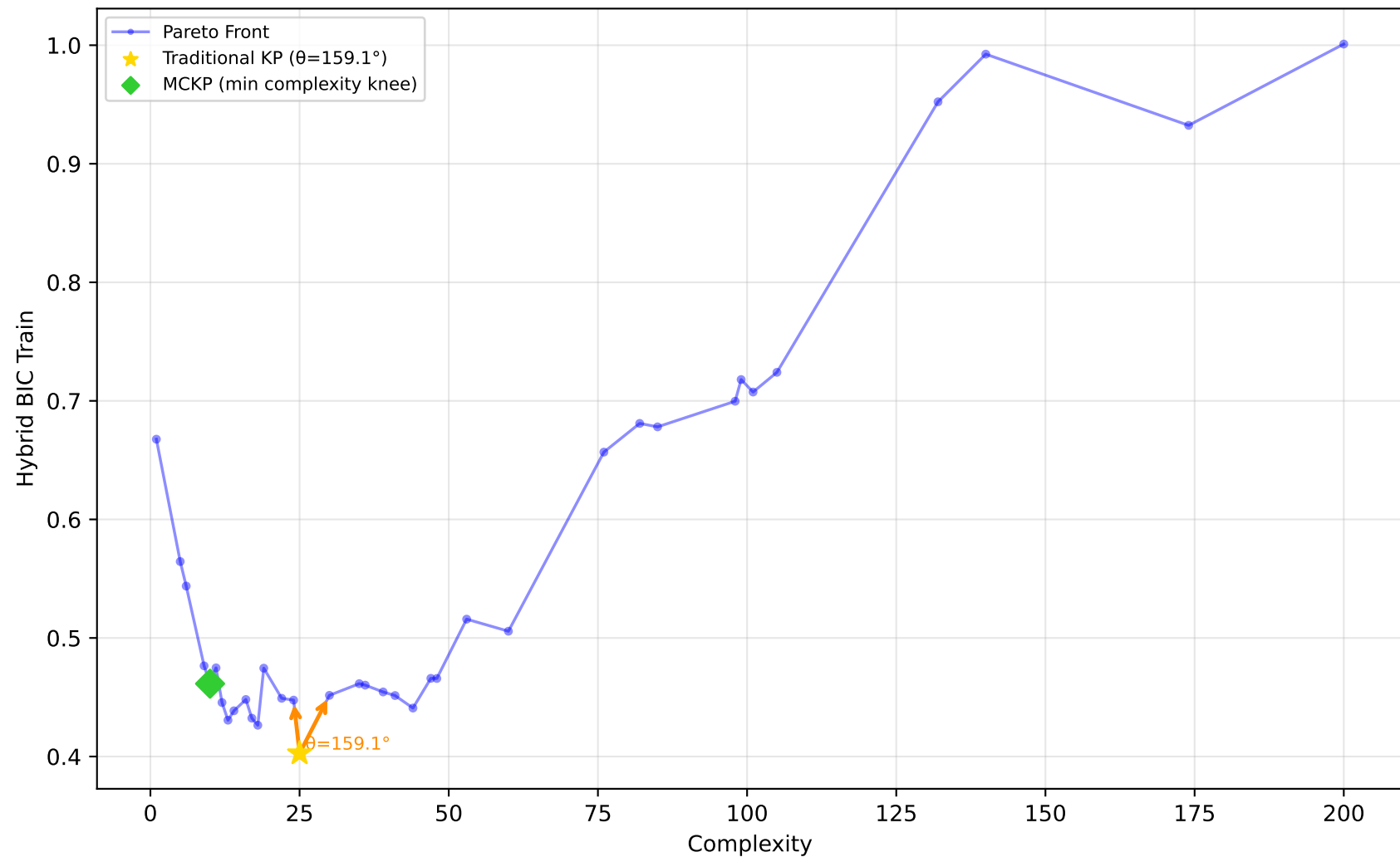
522_pm10 - Run 2 - MVP - Hybrid BIC Train \lambda_1=0.00, \lambda_2=0.90, \lambda_3=0.00 | Difficulty: 1.00 | Method: hmr
