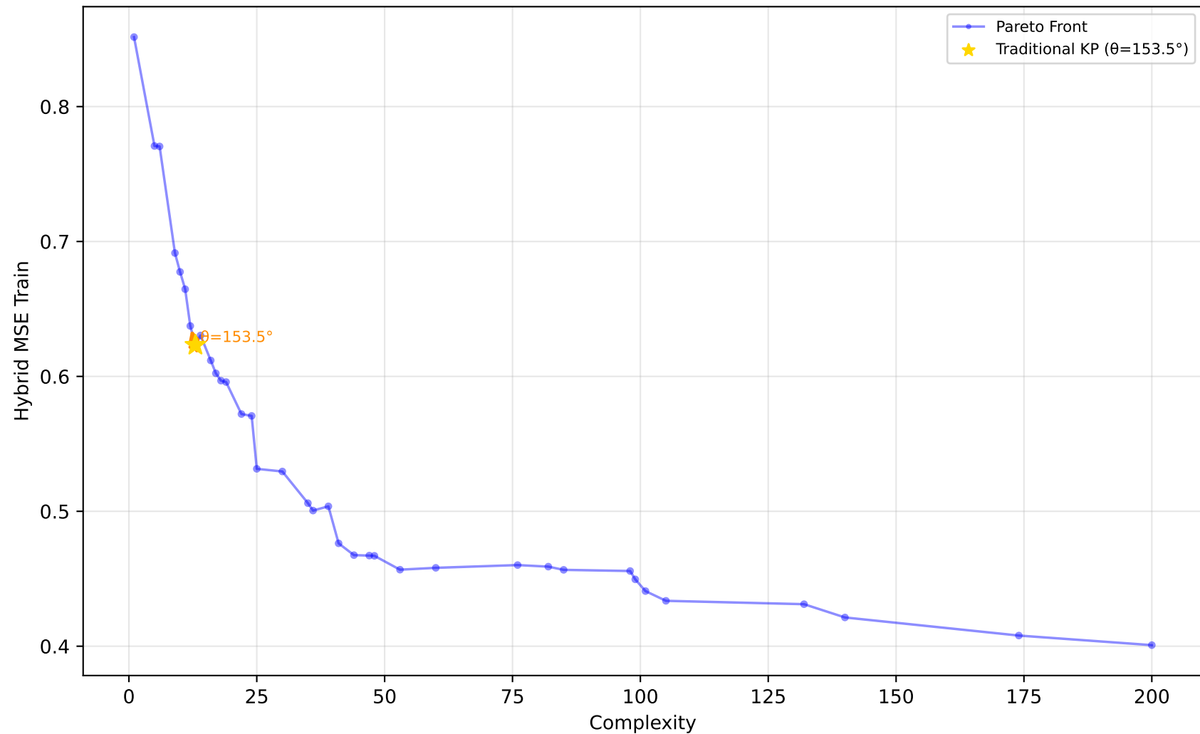
522_pm10 - Run 2 - MVP - Hybrid MSE Train \lambda_1=1.00, \lambda_2=0.00, \lambda_3=0.00 | Difficulty: 1.00 | Method: hmr
