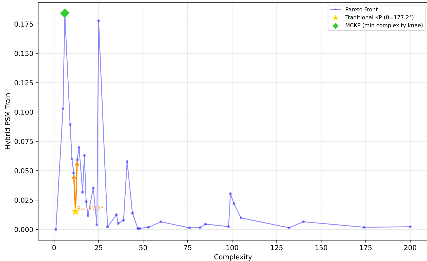
522_pm10 - Run 2 - MVP - Hybrid PSM Train \lambda_1=0.00, \lambda_2=0.90, \lambda_3=0.00 | Difficulty: 1.00 | Method: hmr
