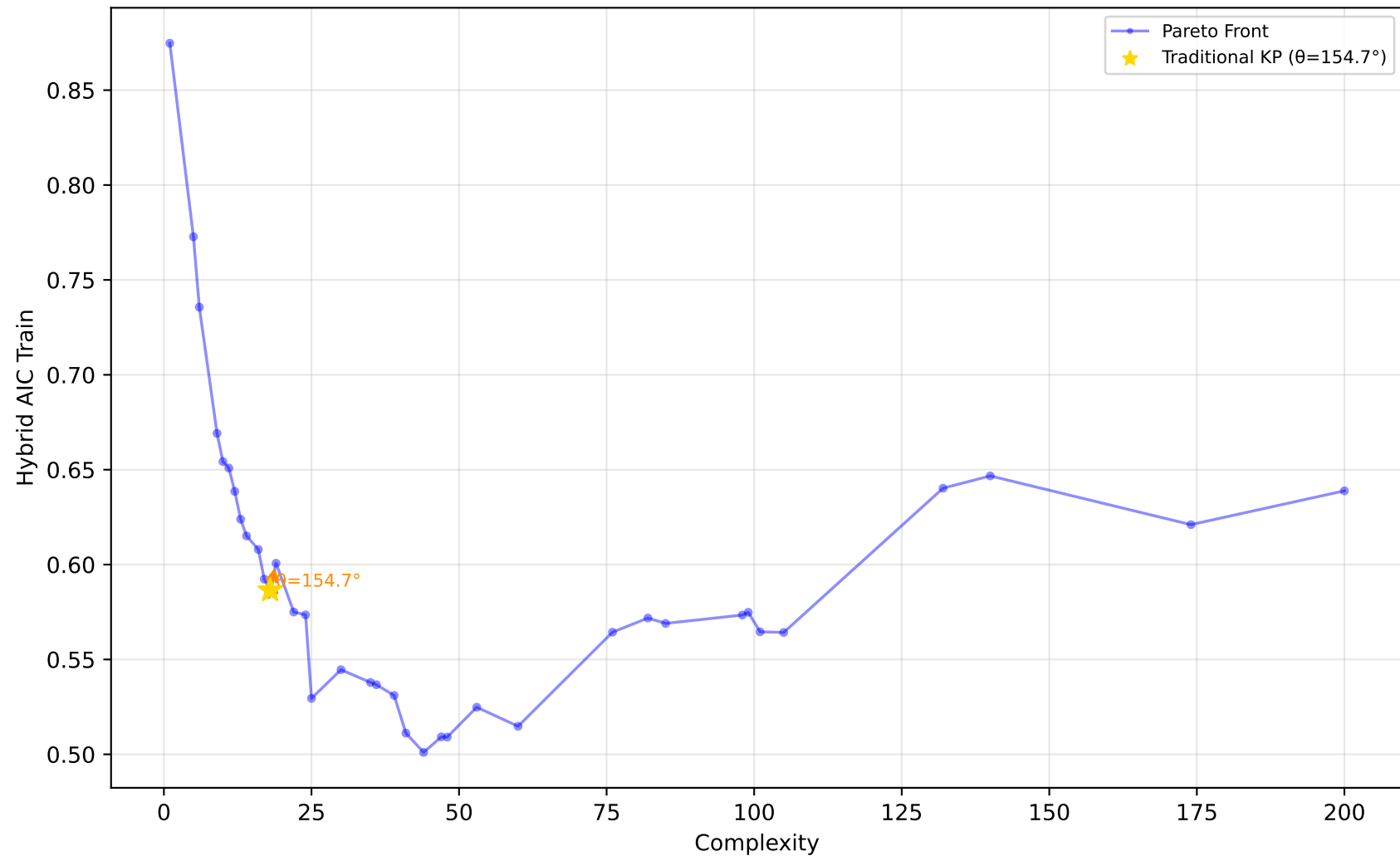
522_pm10 - Run 2 - SVP - Hybrid AIC Train \lambda_1=0.00, \lambda_2=0.10, \lambda_3=0.00 | Difficulty: 1.00 | Method: hmr
