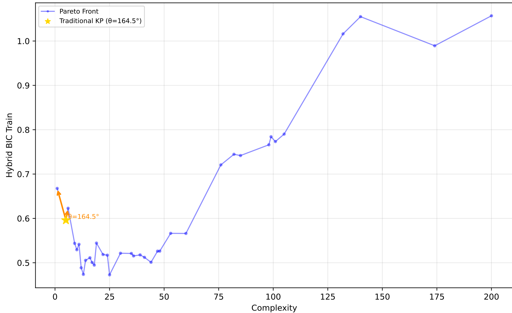
522_pm10 - Run 2 - SVP - Hybrid BIC Train \lambda_1=1.00, \lambda_2=0.00, \lambda_3=0.90 | Difficulty: 1.00 | Method: hmr
