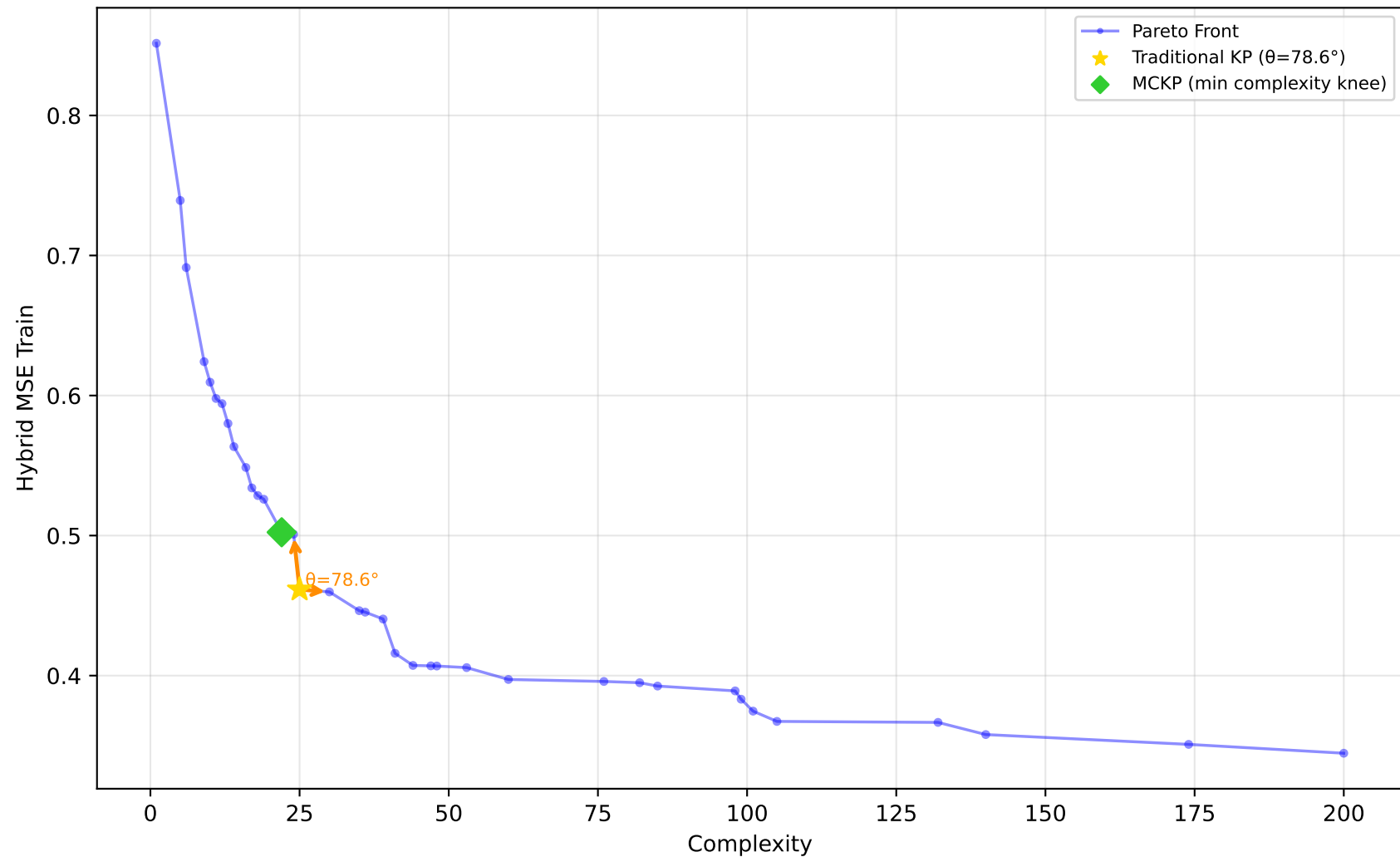
522_pm10 - Run 2 - SVP - Hybrid MSE Train \lambda_1=0.00, \lambda_2=0.10, \lambda_3=0.00 | Difficulty: 1.00 | Method: hmr
