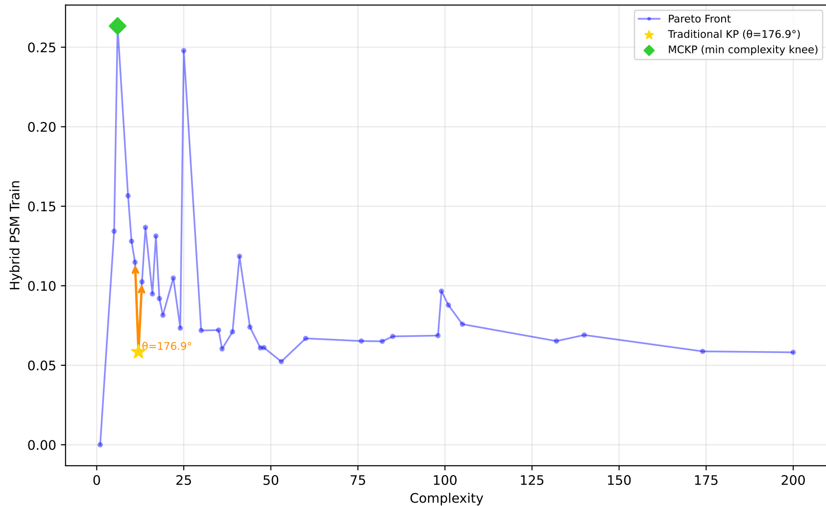
522_pm10 - Run 2 - SVP - Hybrid PSM Train \lambda_1=1.00, \lambda_2=0.00, \lambda_3=0.90 | Difficulty: 1.00 | Method: hmr
