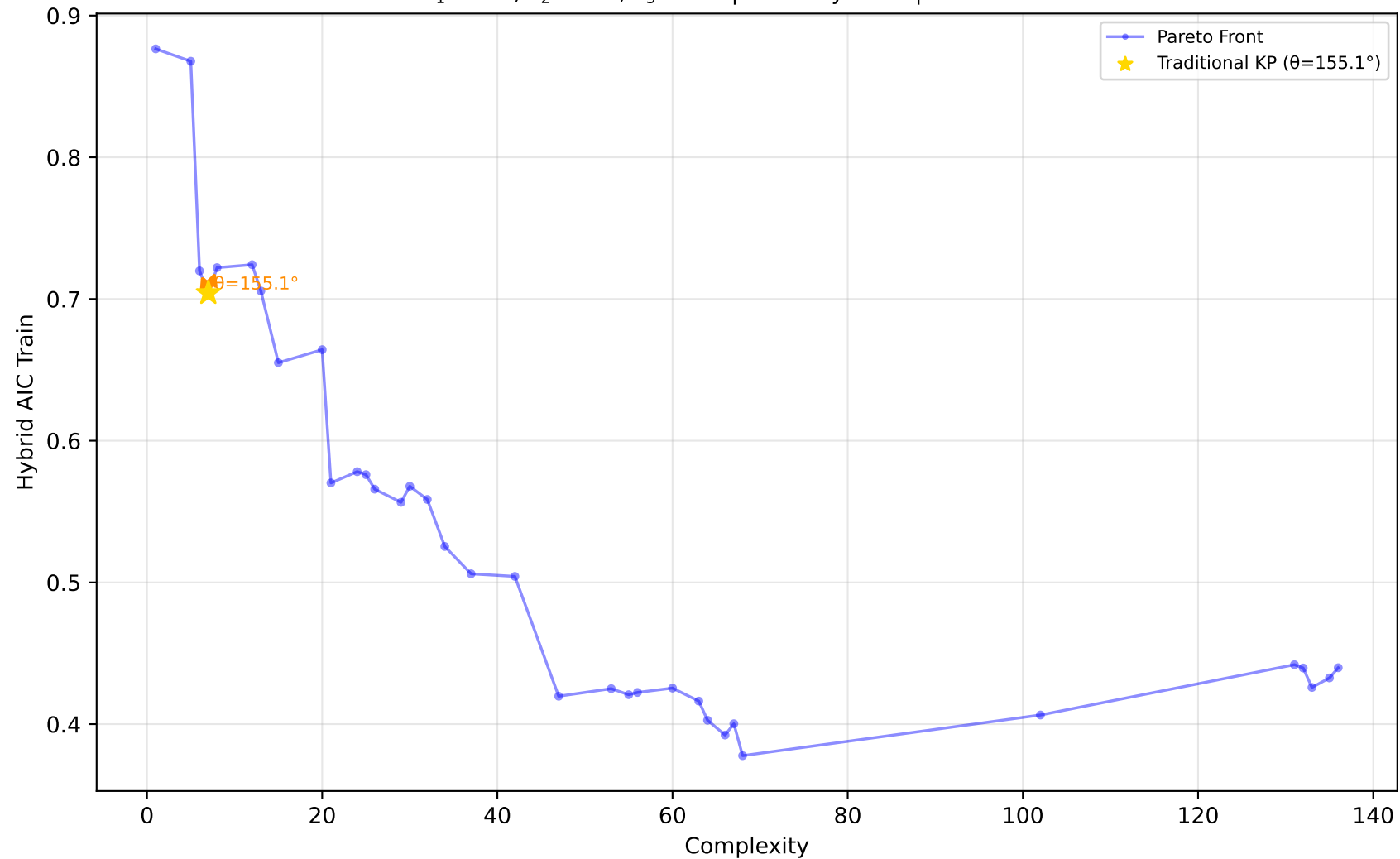
522_pm10 - Run 30 - MVP - Hybrid AIC Train \lambda_1=1.00, \lambda_2=0.00, \lambda_3=0.00 | Difficulty: 1.00 | Method: hmr
