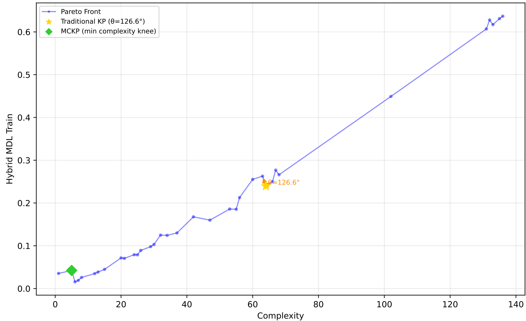
522_pm10 - Run 30 - MVP - Hybrid MDL Train \lambda_1=0.00, \lambda_2=0.90, \lambda_3=0.00 | Difficulty: 1.00 | Method: hmr
