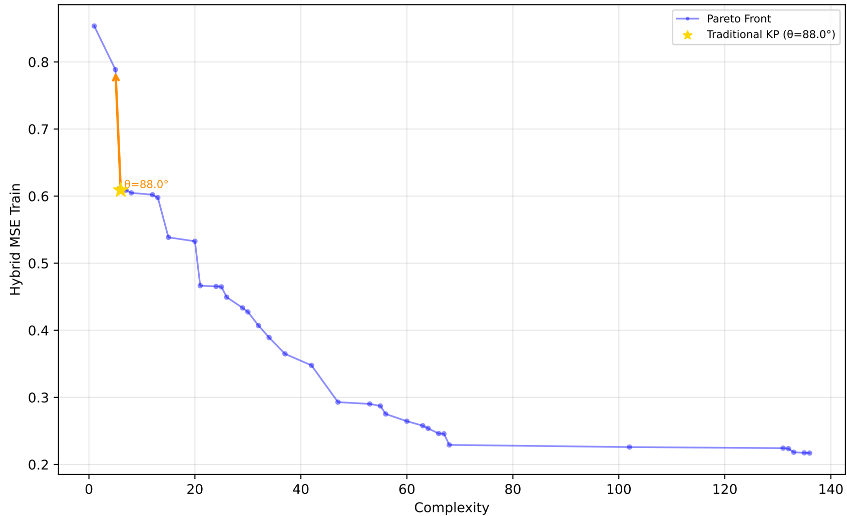
522_pm10 - Run 30 - MVP - Hybrid MSE Train \lambda_1=0.00, \lambda_2=0.90, \lambda_3=0.00 | Difficulty: 1.00 | Method: hmr
