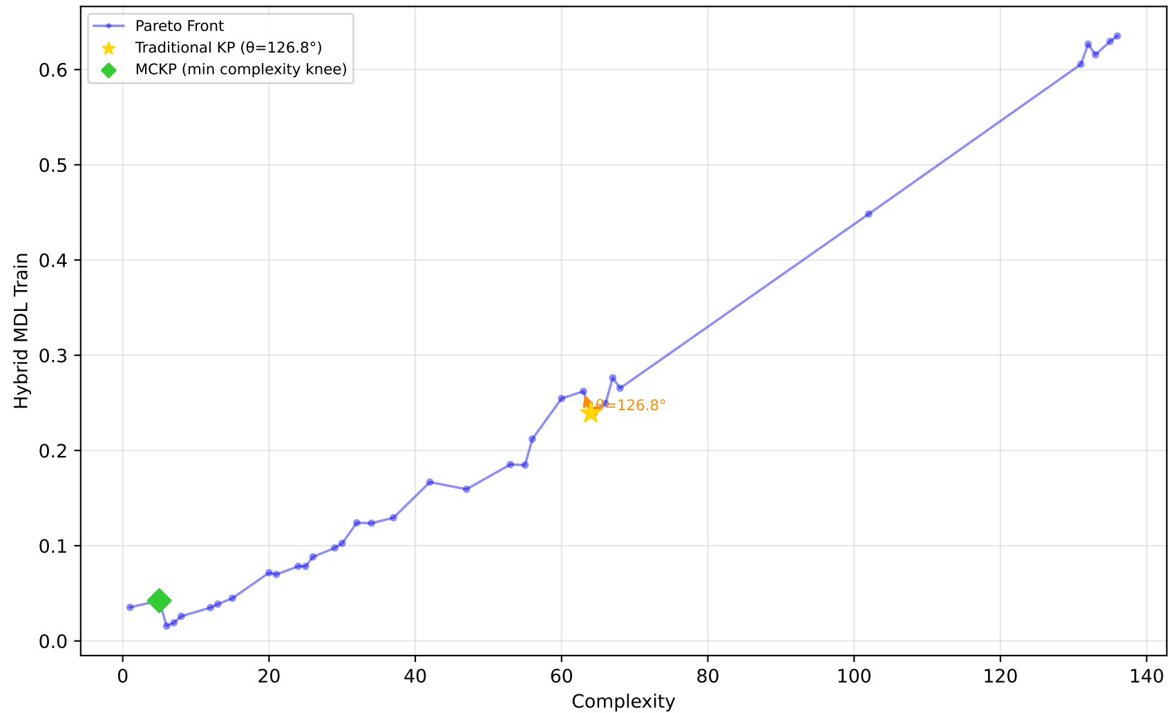
522_pm10 - Run 30 - SVP - Hybrid MDL Train \lambda_1=0.00, \lambda_2=0.10, \lambda_3=0.00 | Difficulty: 1.00 | Method: hmr
