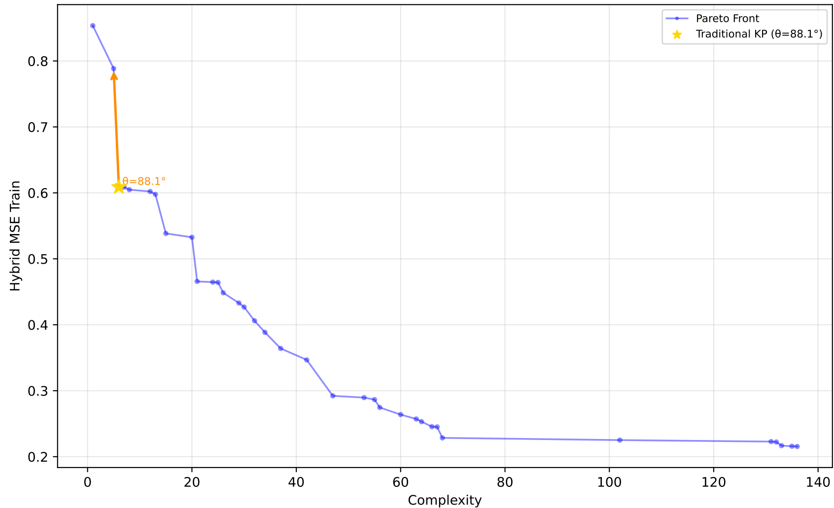
522_pm10 - Run 30 - SVP - Hybrid MSE Train \lambda_1=0.00, \lambda_2=0.10, \lambda_3=0.00 | Difficulty: 1.00 | Method: hmr
